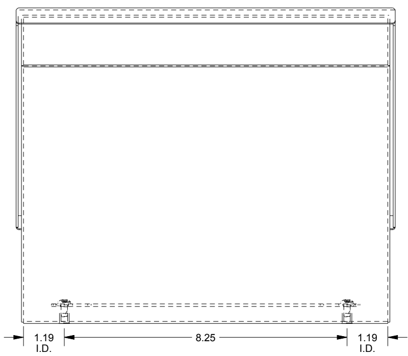
REAR VIEW
