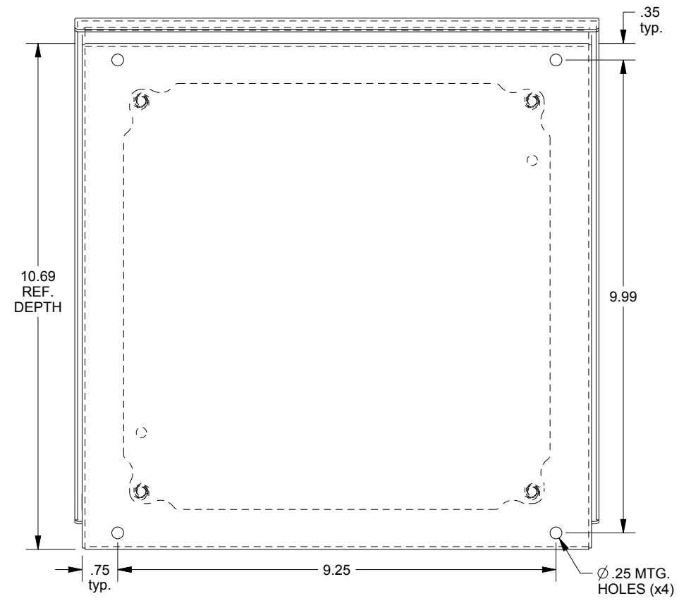
BOTTOM VIEW
