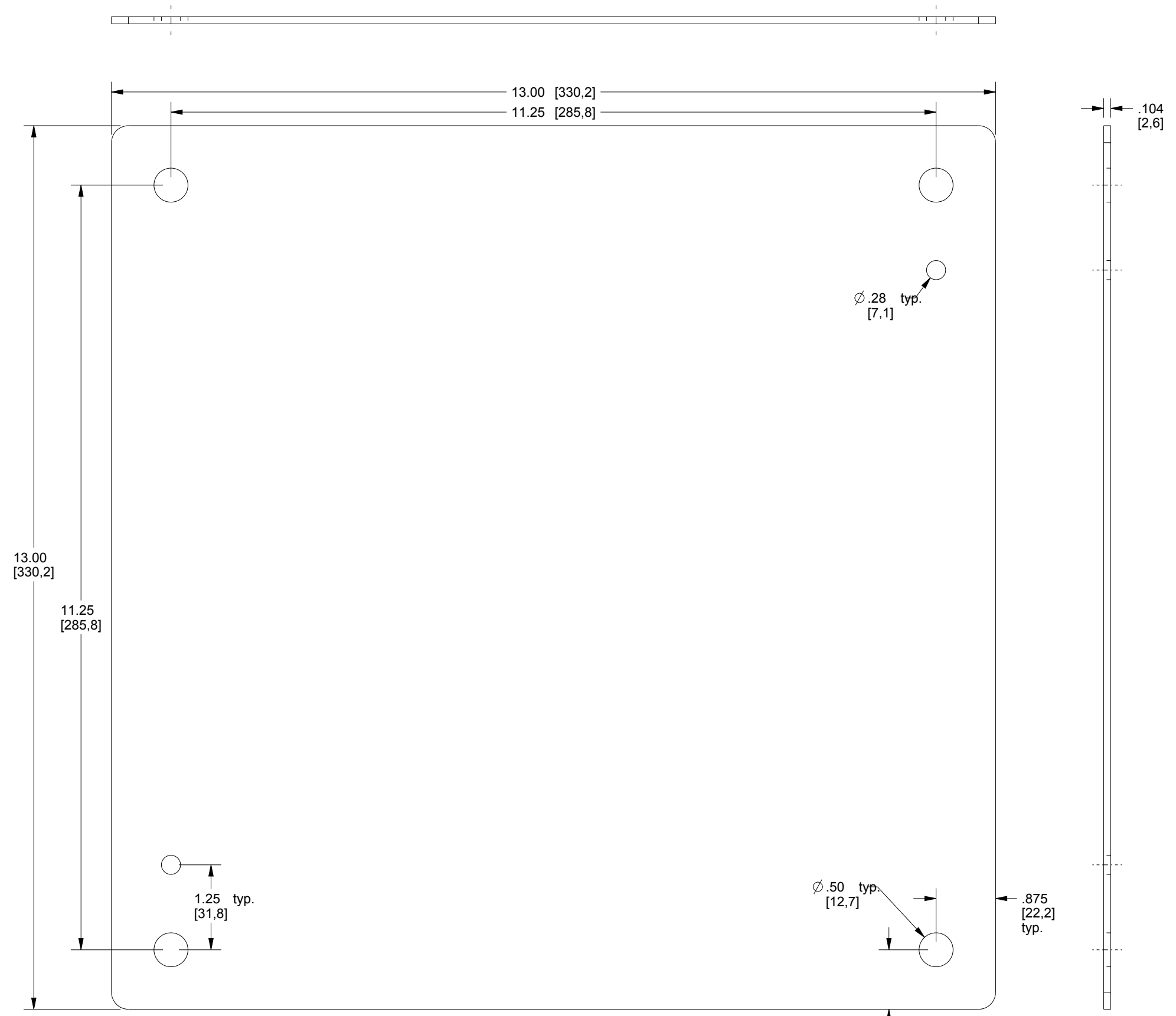
SUBPANEL FRONT VIEW
