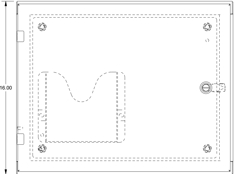
FRONT VIEW
