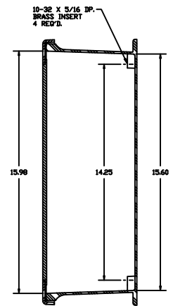
SECTION B-B
