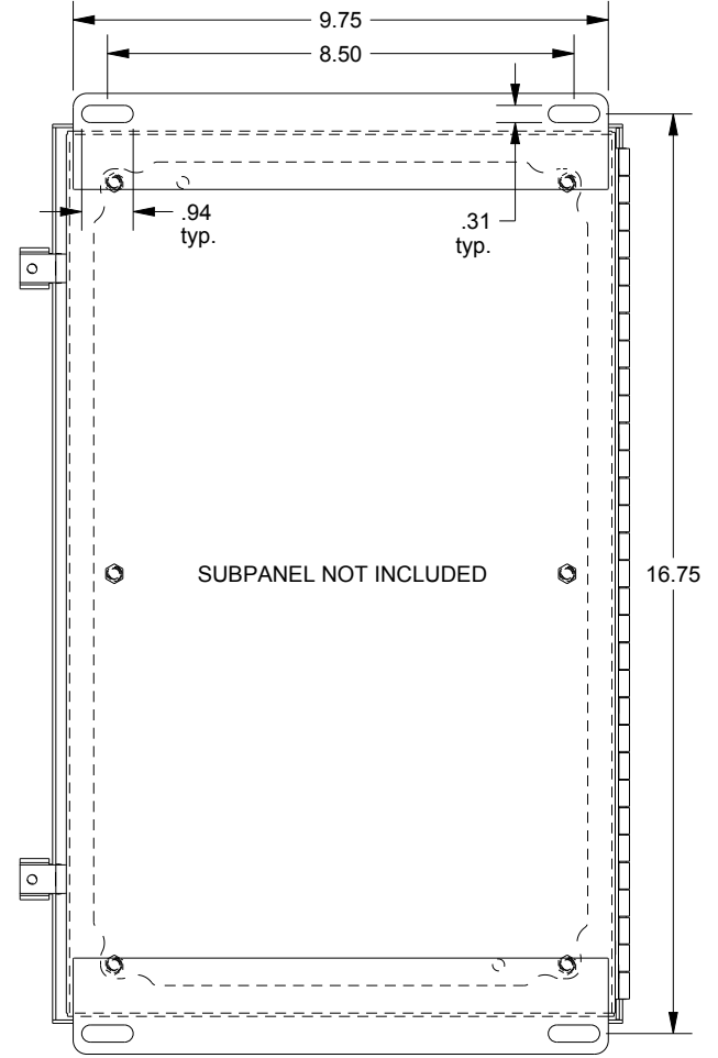
EXTERNAL REAR VIEW
