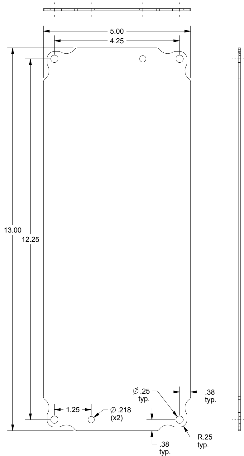
SUBPANEL FRONT VIEW
