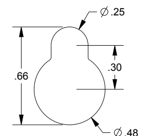
MOUNTING HOLE DETAIL (4plcs.)
