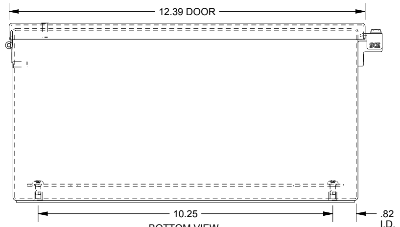
BOTTOM VIEW
