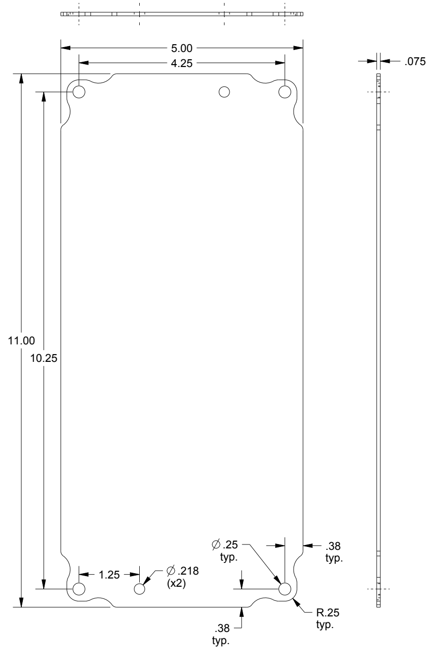
SUBPANEL FRONT VIEW
