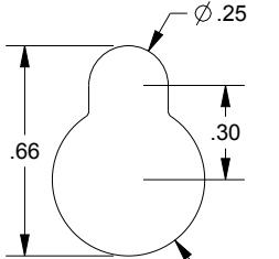
MOUNTING HOLE DETAIL (4plcs.)
