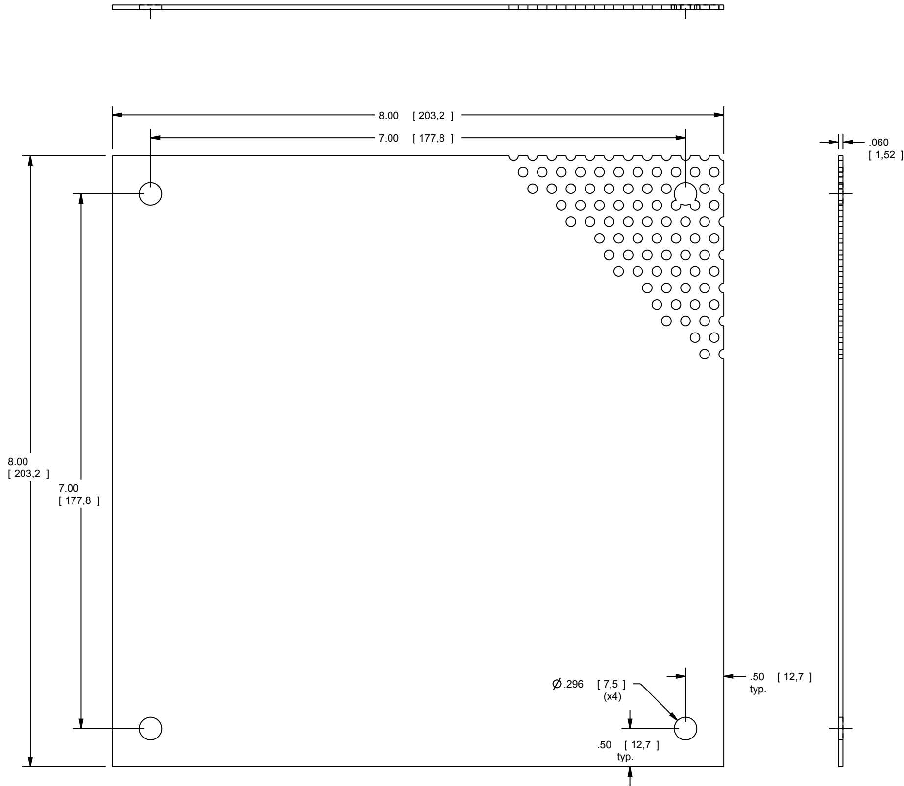
SUBPANEL FRONT VIEW
