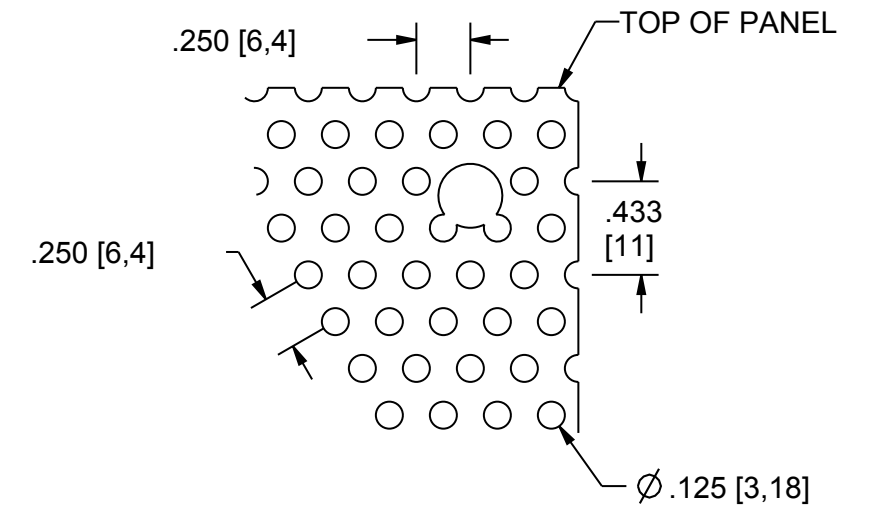
PERFORATED PATTERN DETAIL
