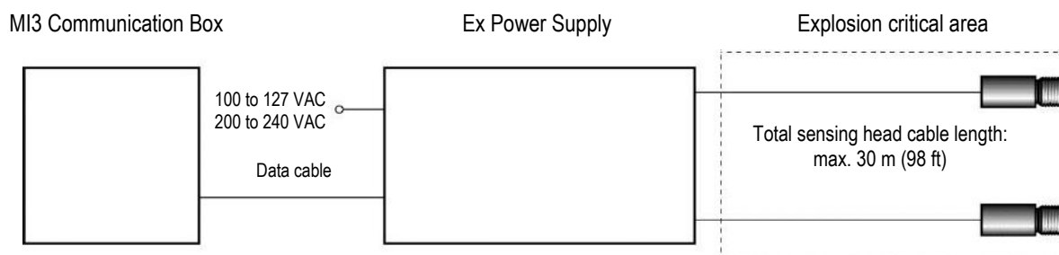
Figure 42: Basic Installation in the Explosion Critical Area
