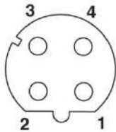
Figure 87: M12 Connector Socket and Pin Assignment
