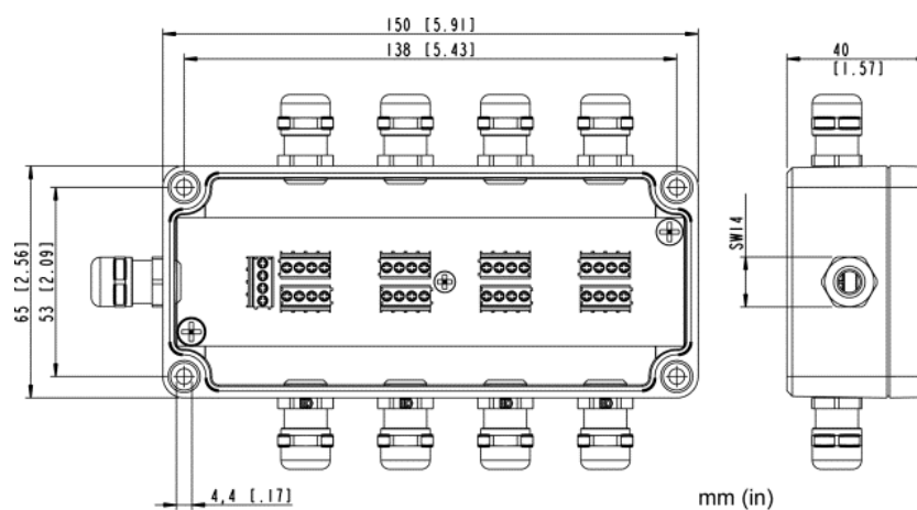
Figure 48: Dimensions
