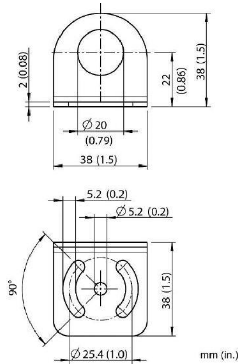
Figure 69: Dimensions of Fixed Mounting Bracket (XXXMI3100FB)
