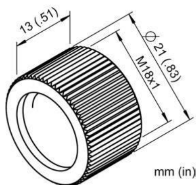
Figure 75: Protective Window
