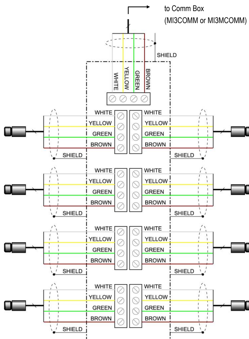
Figure 49: Wiring Diagram for 8 Heads
