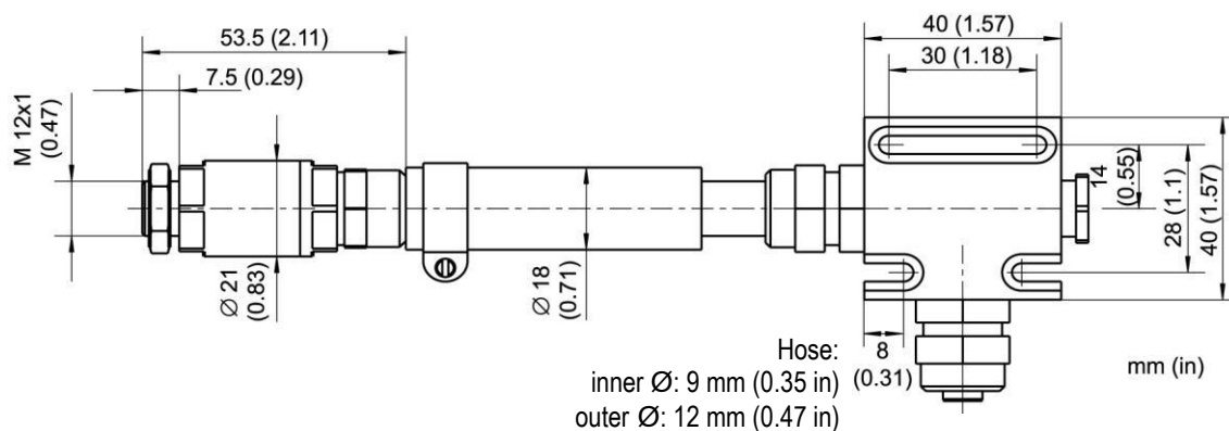
Figure 62: Dimensions of Air Cooling System
