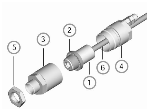
Figure 57: Mounting the Air Purge Jacket
