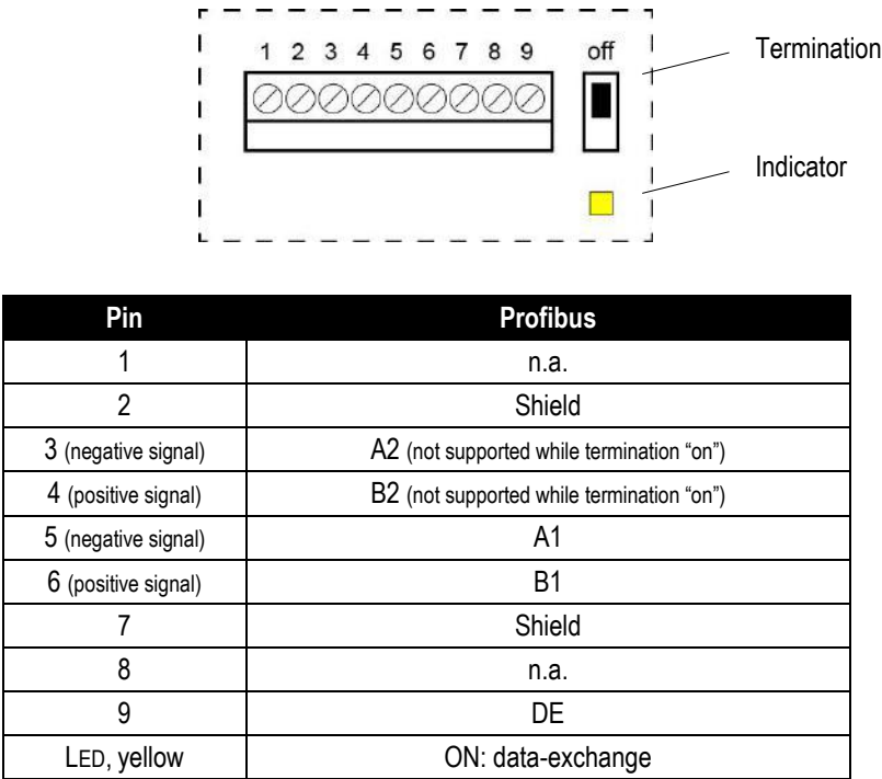
Figure 82: Terminal for Comm Box (DIN 6TE)
