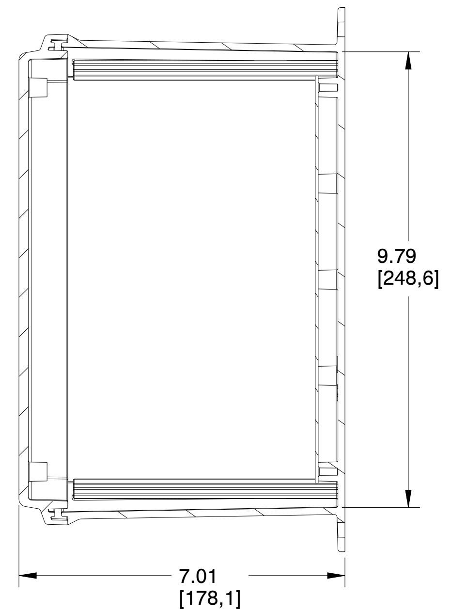
SECTION B-B
