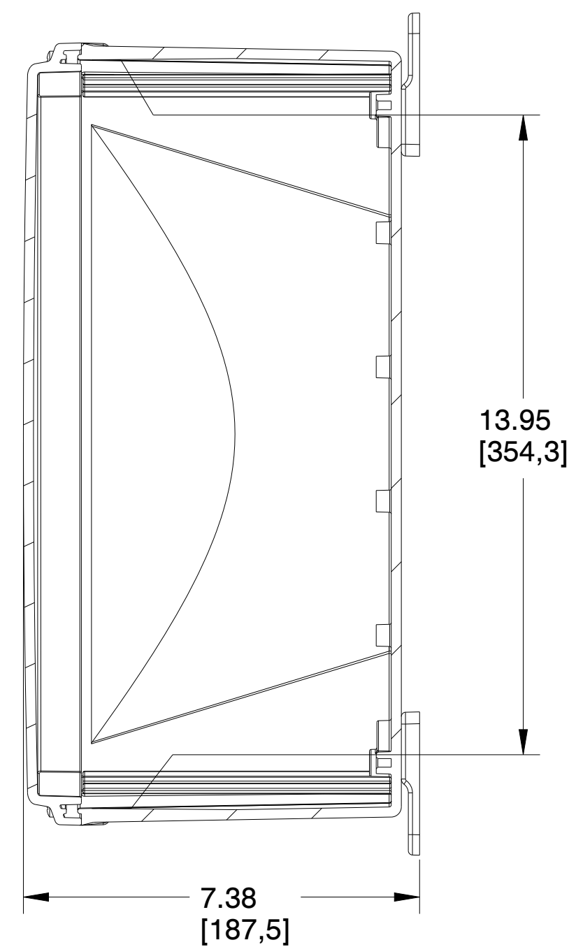
SECTION C-C
