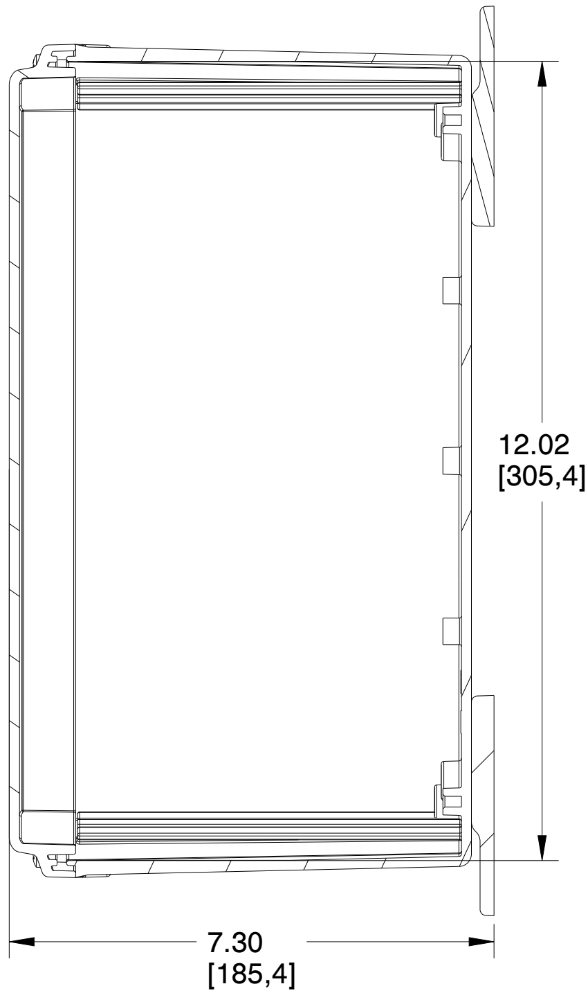
SECTION B-B
