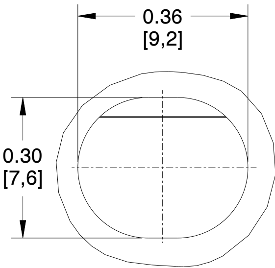
DETAIL A SCALE 5.000 4X PLACES
