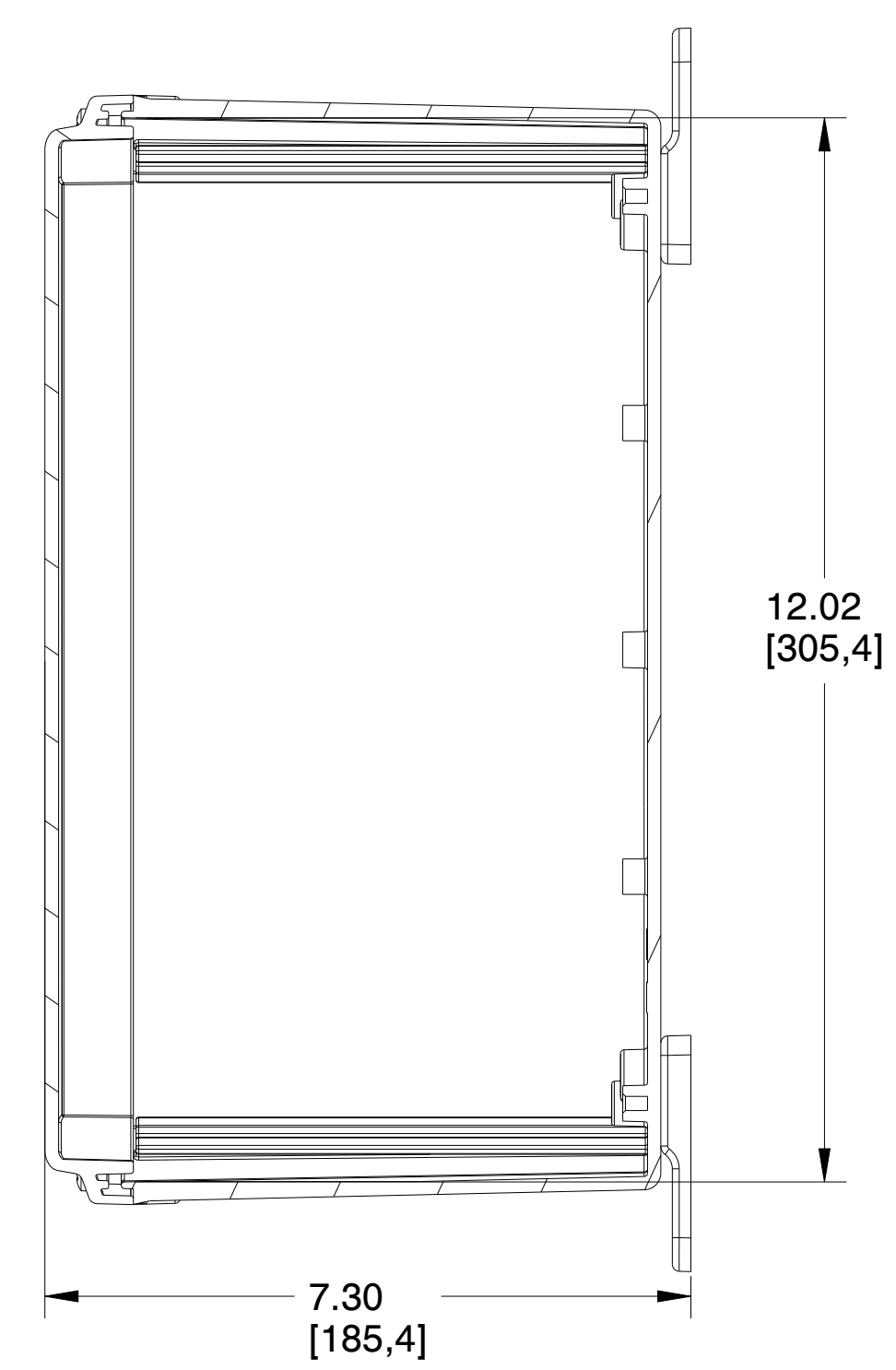
SECTION B-B
