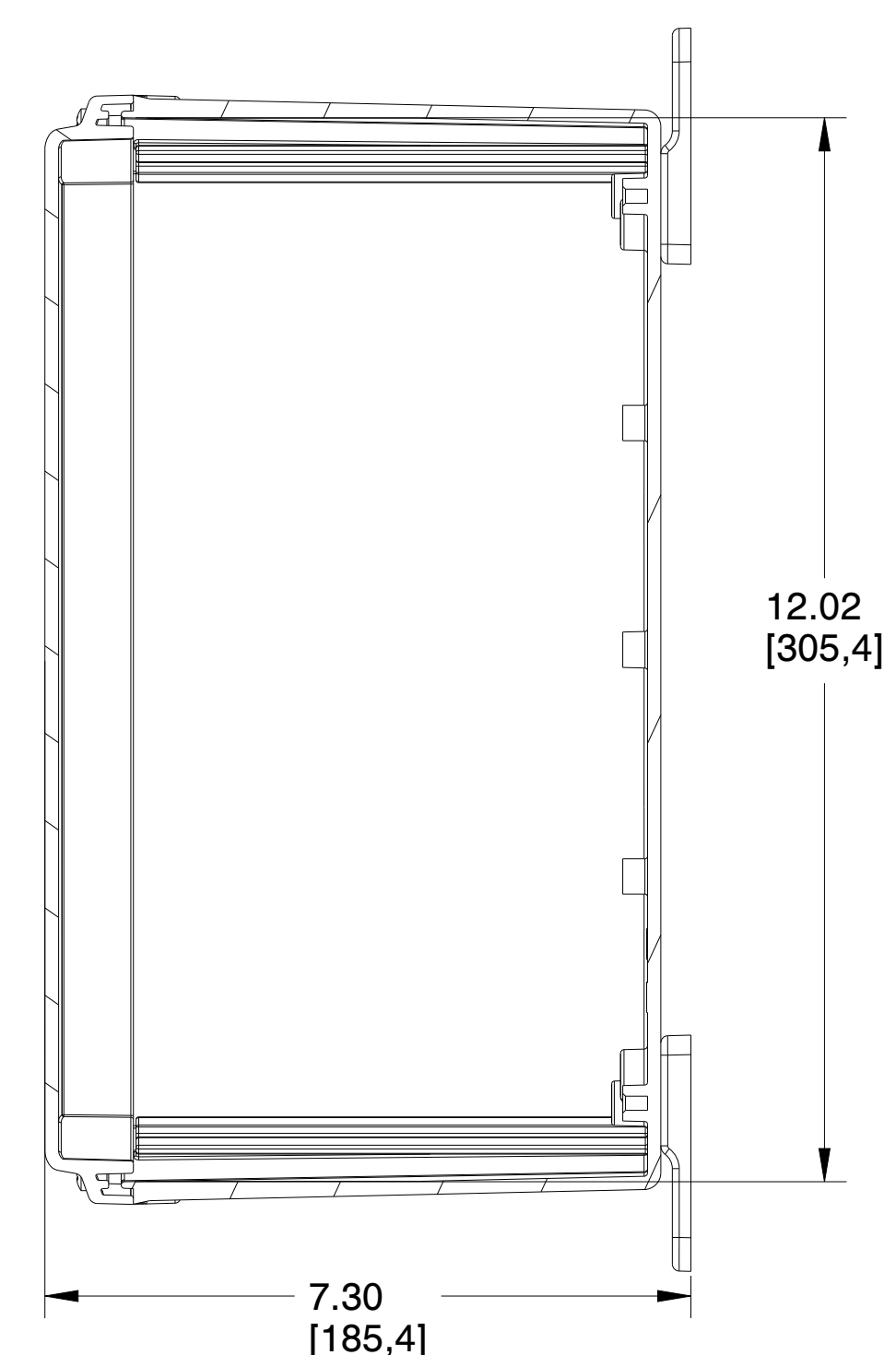
SECTION B-B
