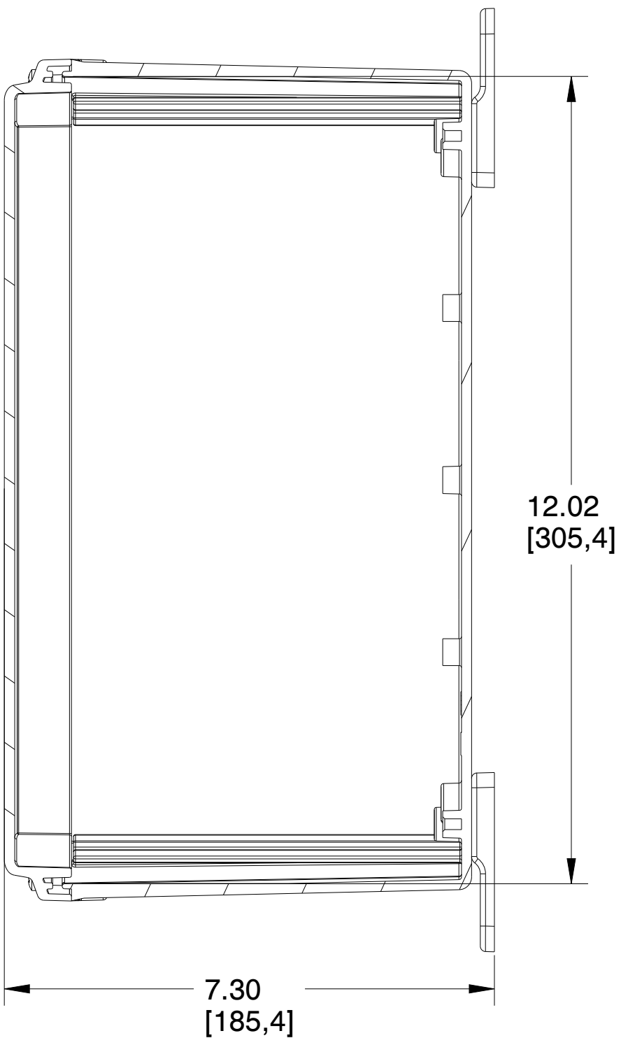
SECTION B-B
