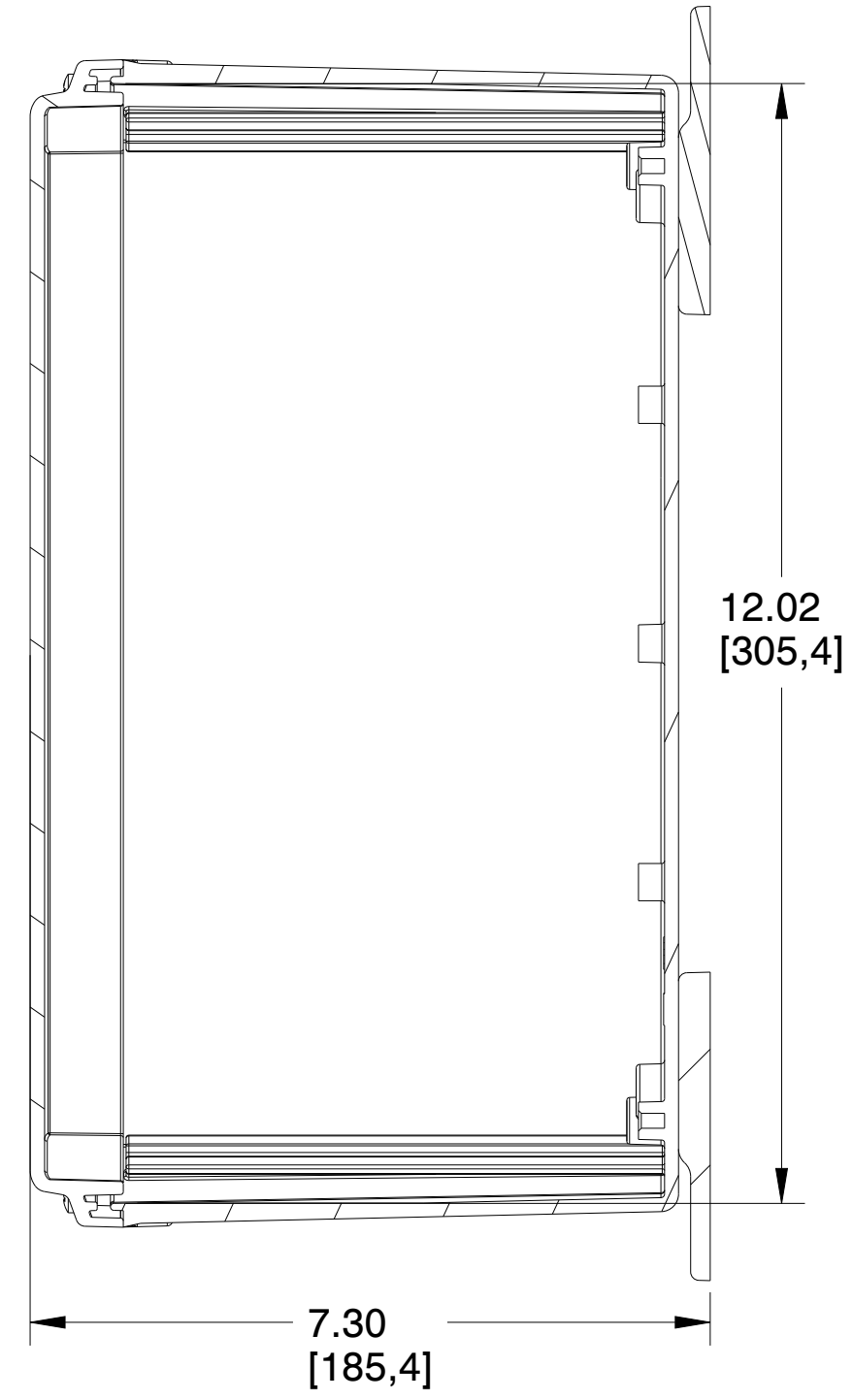
SECTION B-B
