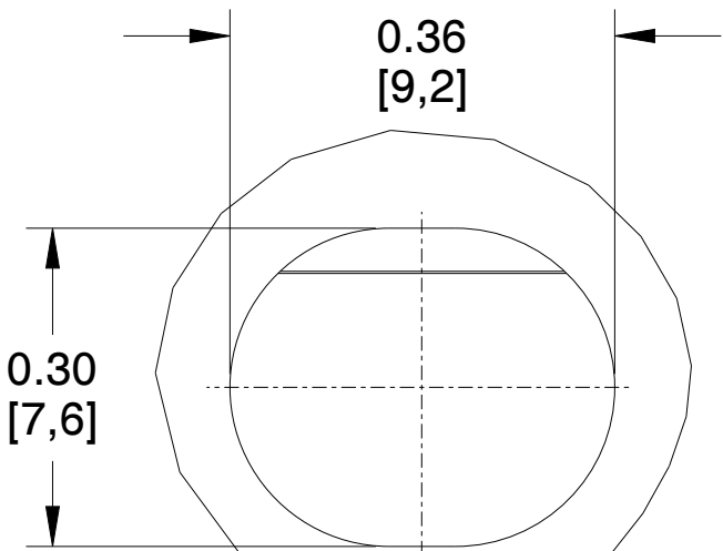
DETAIL A SCALE 5.000 4X PLACES
