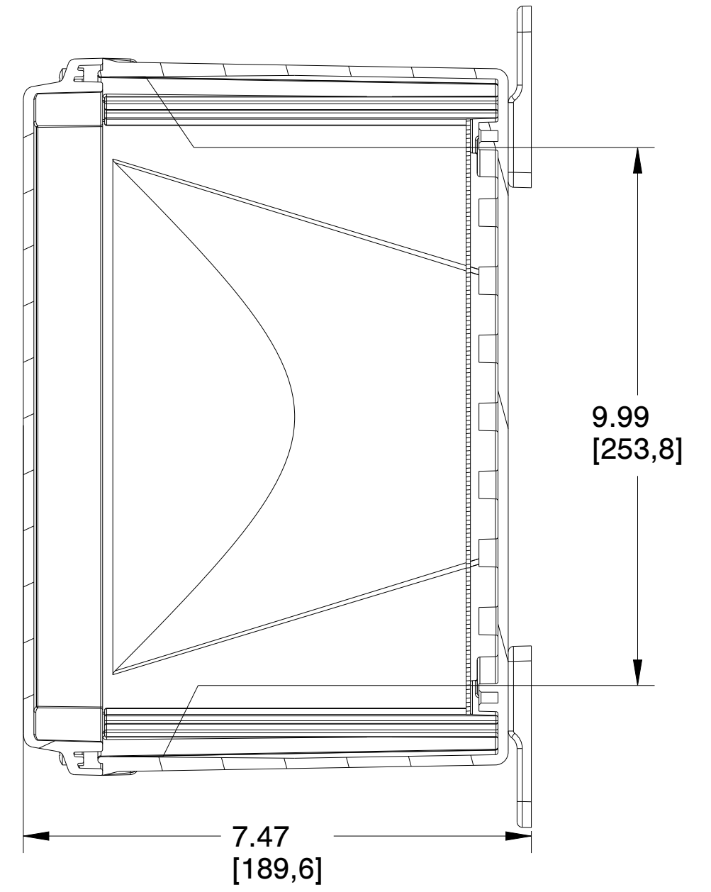
SECTION B-B
