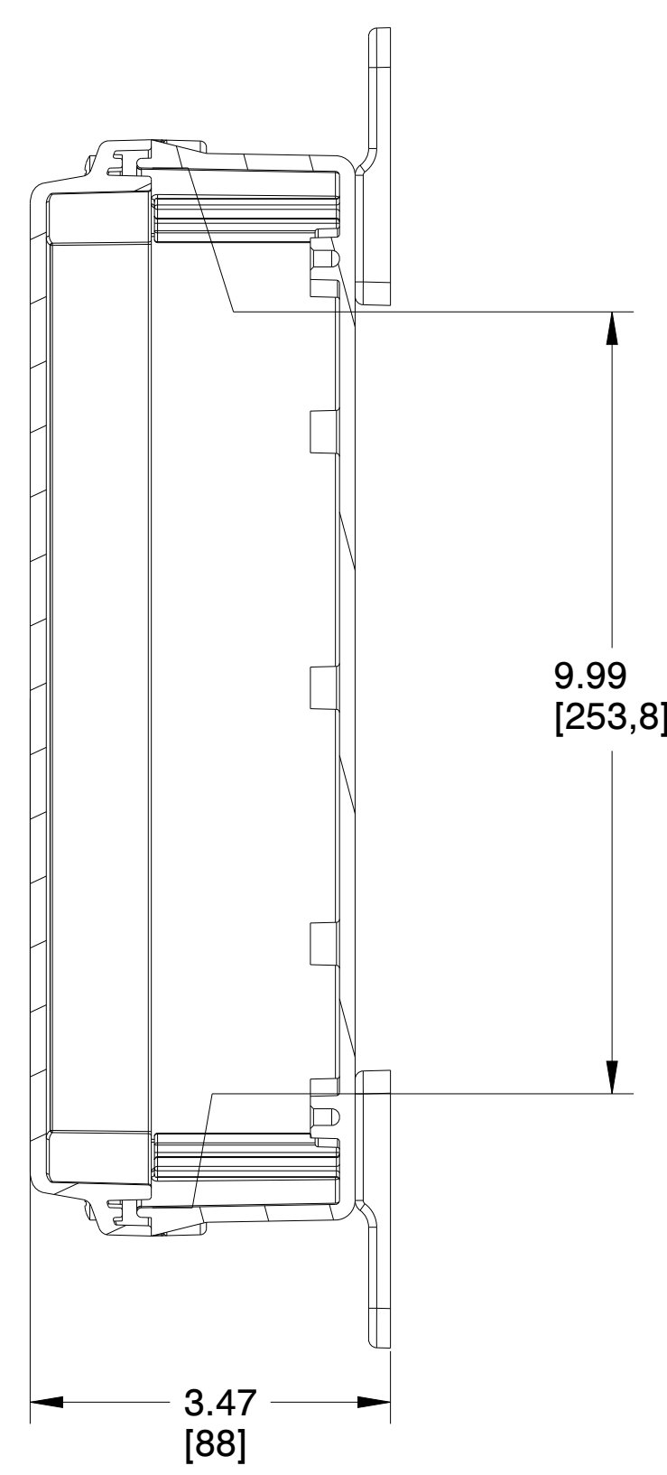
SECTION B-B
