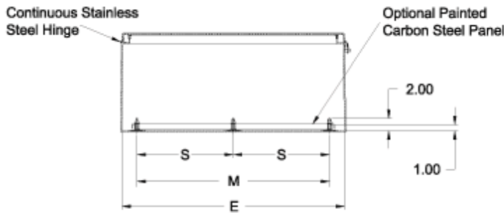
End View
