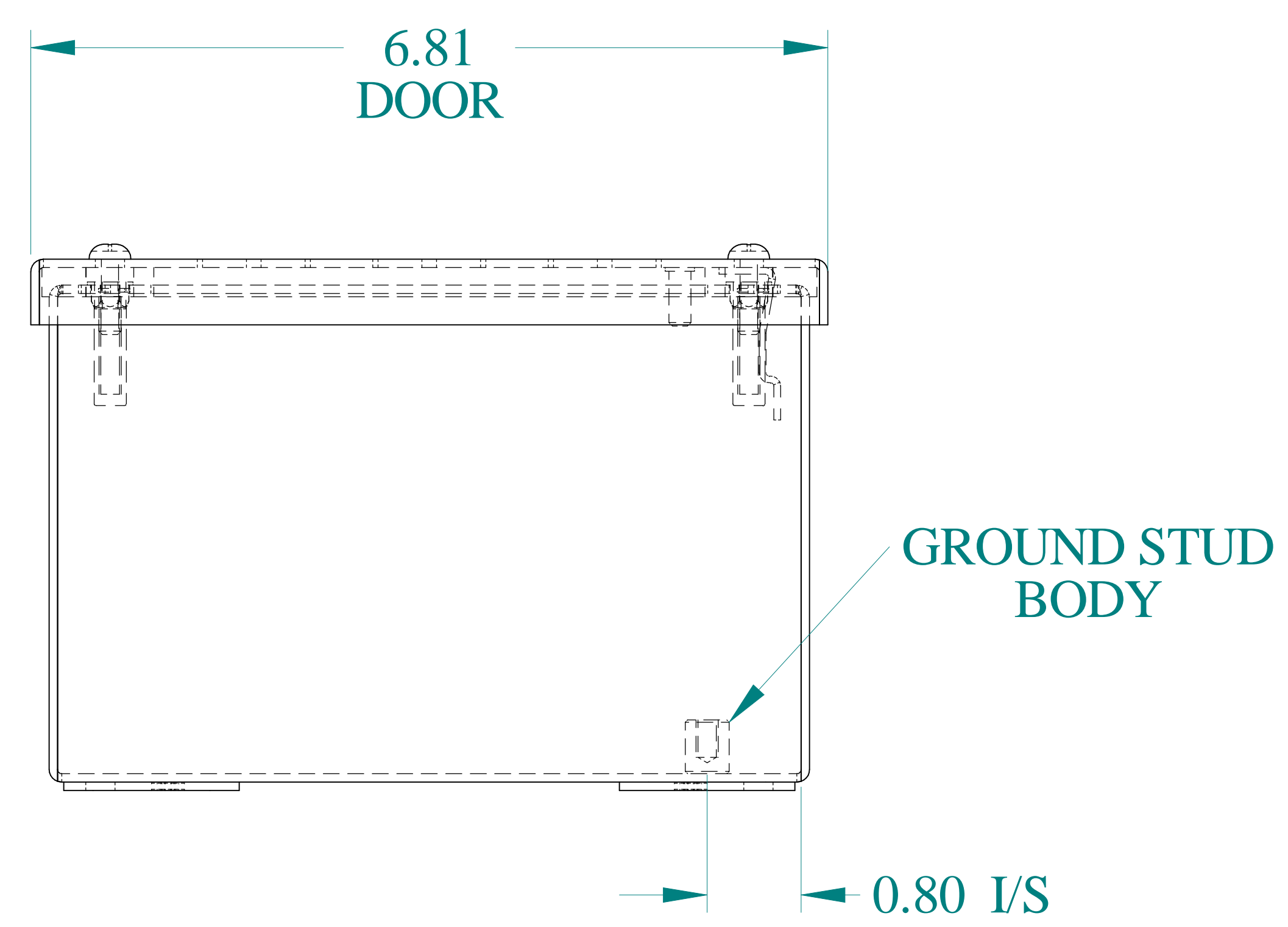
BOTTOM VIEW
