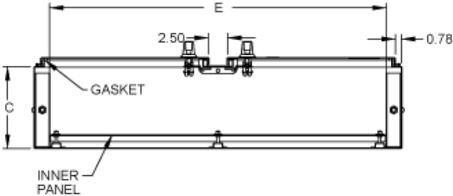
SECTION X-X
