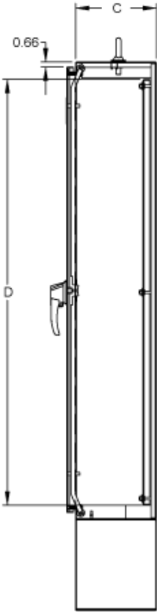
SECTION Y-Y
