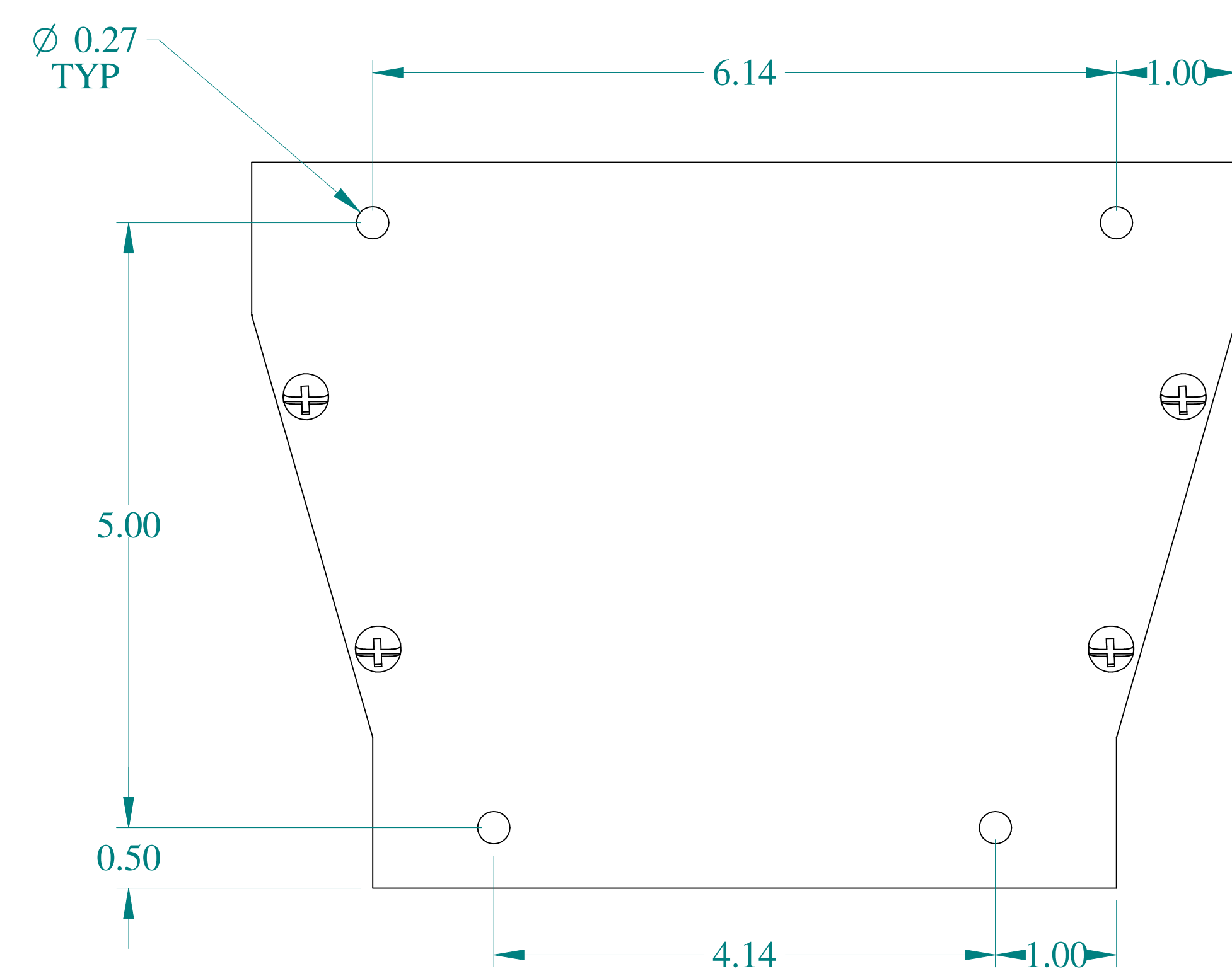
TOP VIEW
