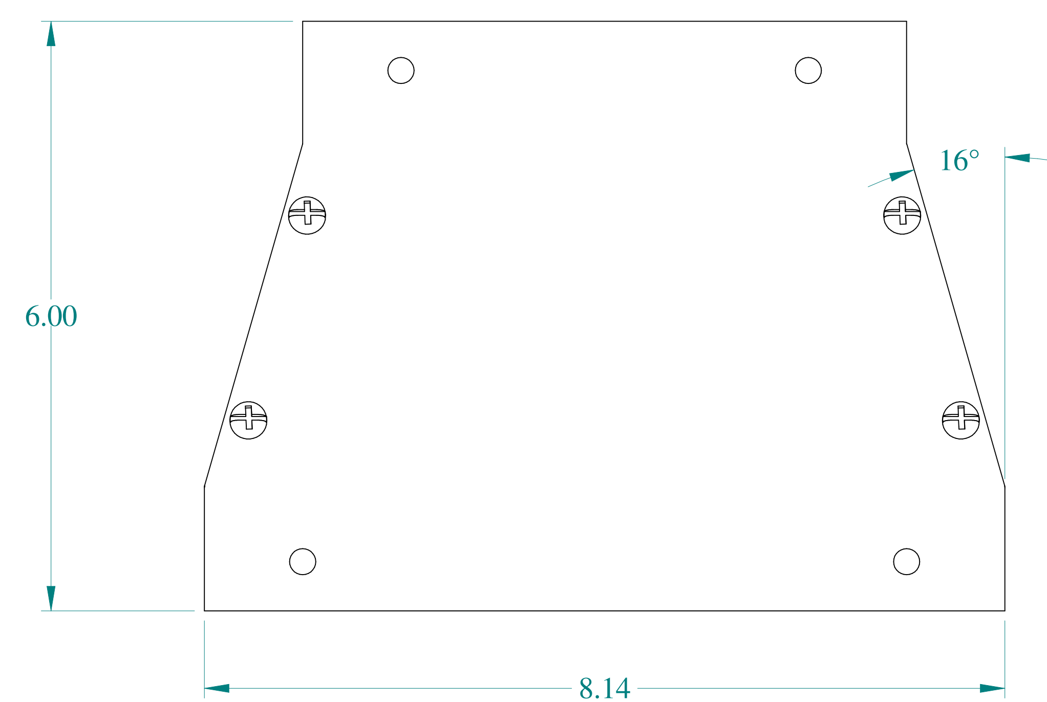
BOTTOM VIEW
