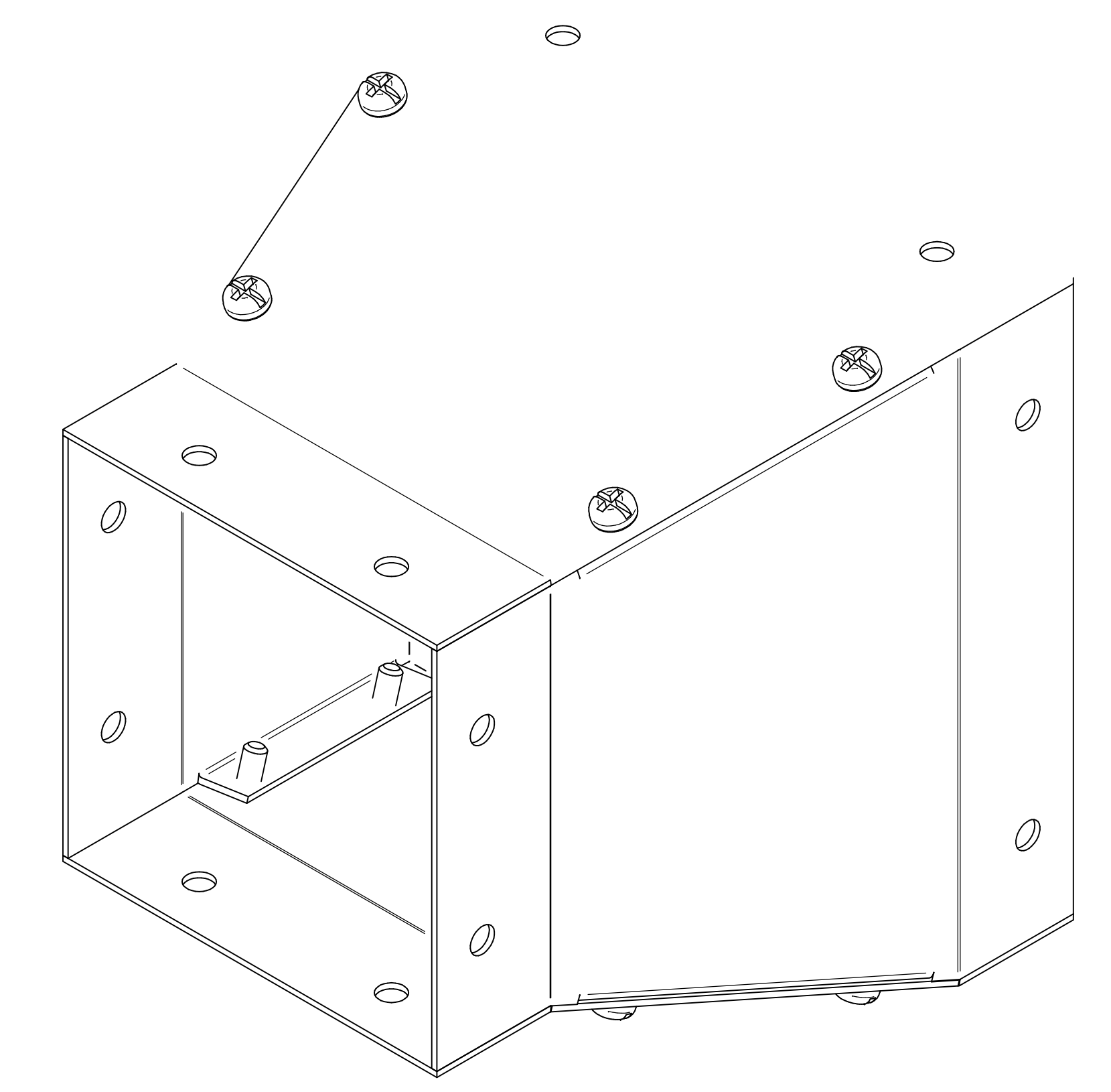
ISOMETRIC VIEWS
