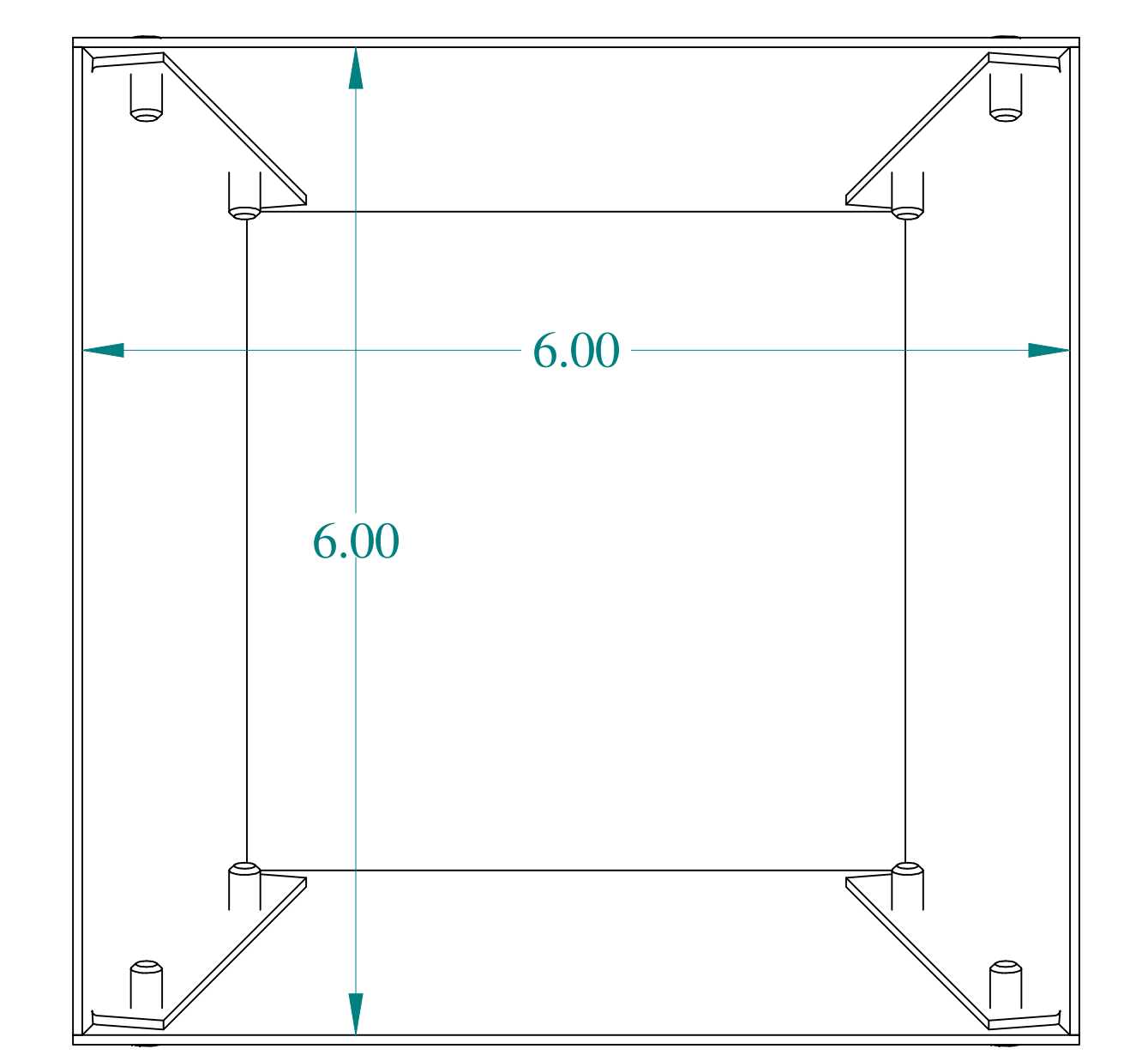
BACK VIEW
