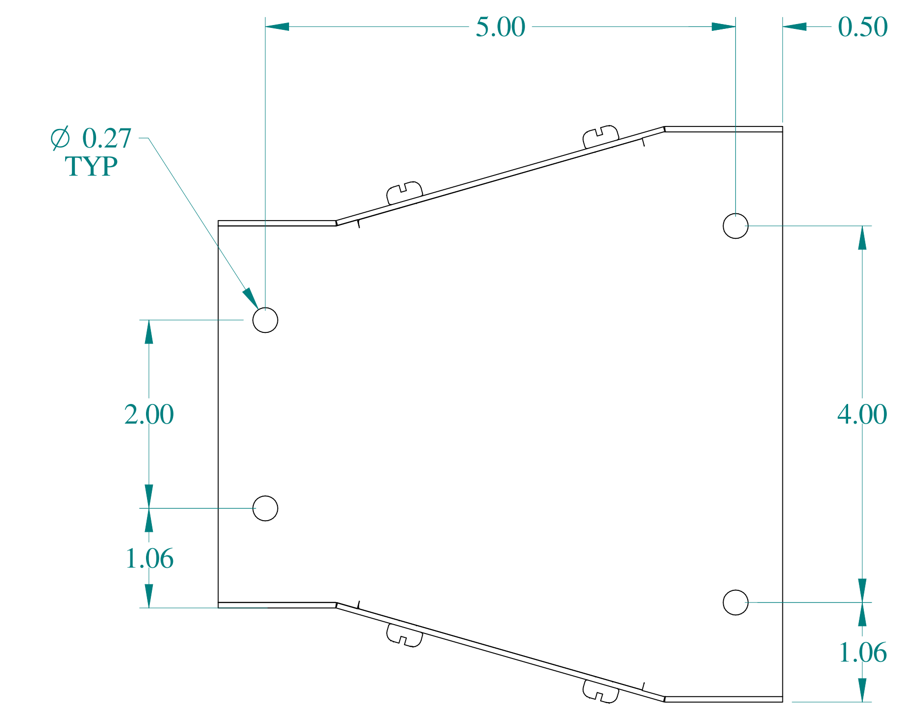
SIDE VIEW
