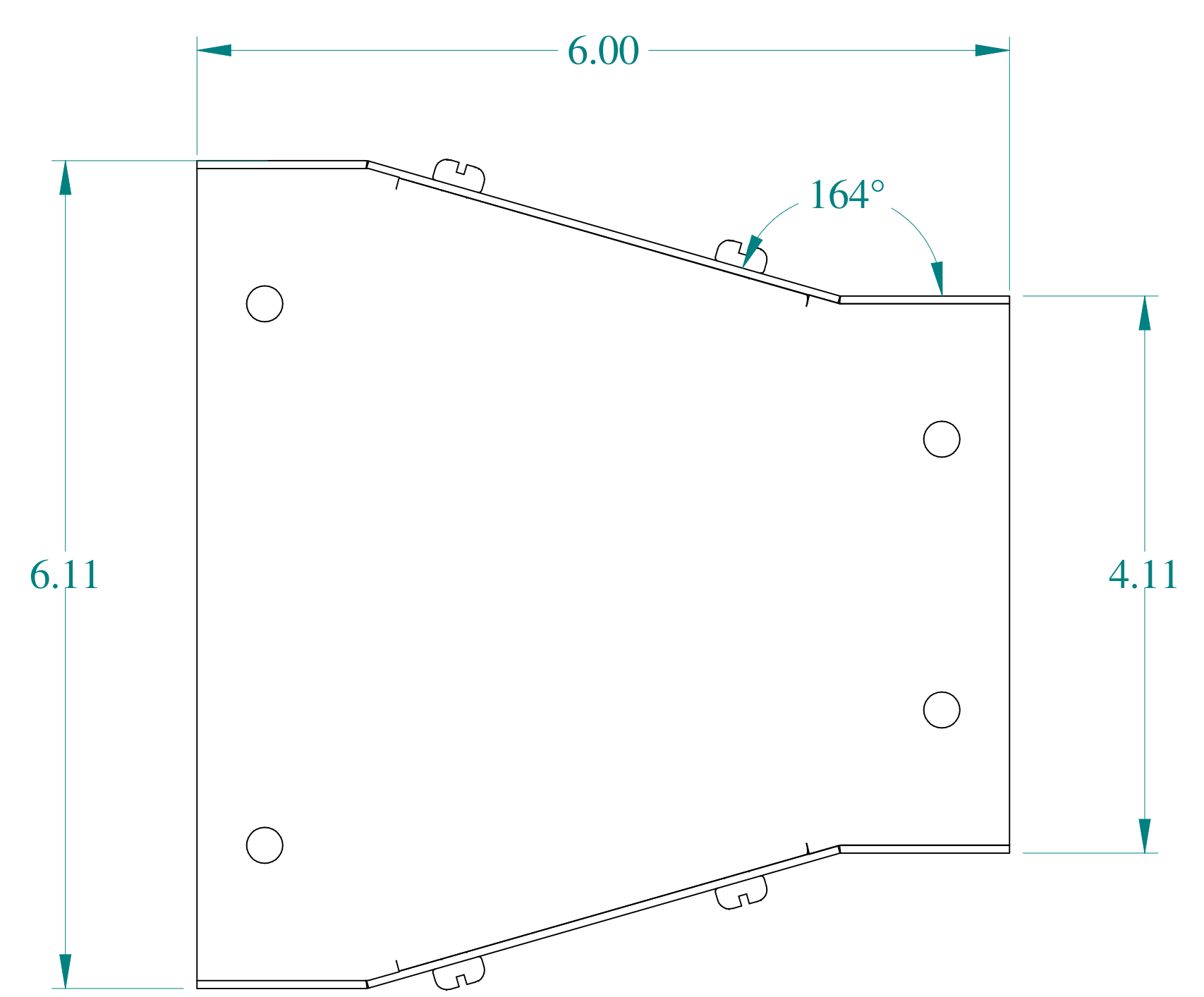
SIDE VIEW
