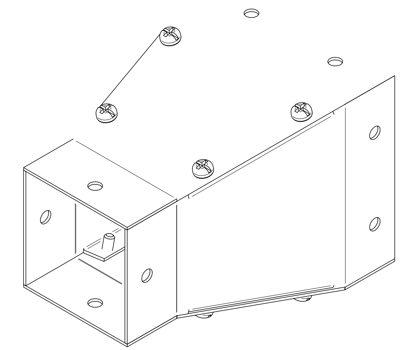
ISOMETRIC VIEWS
