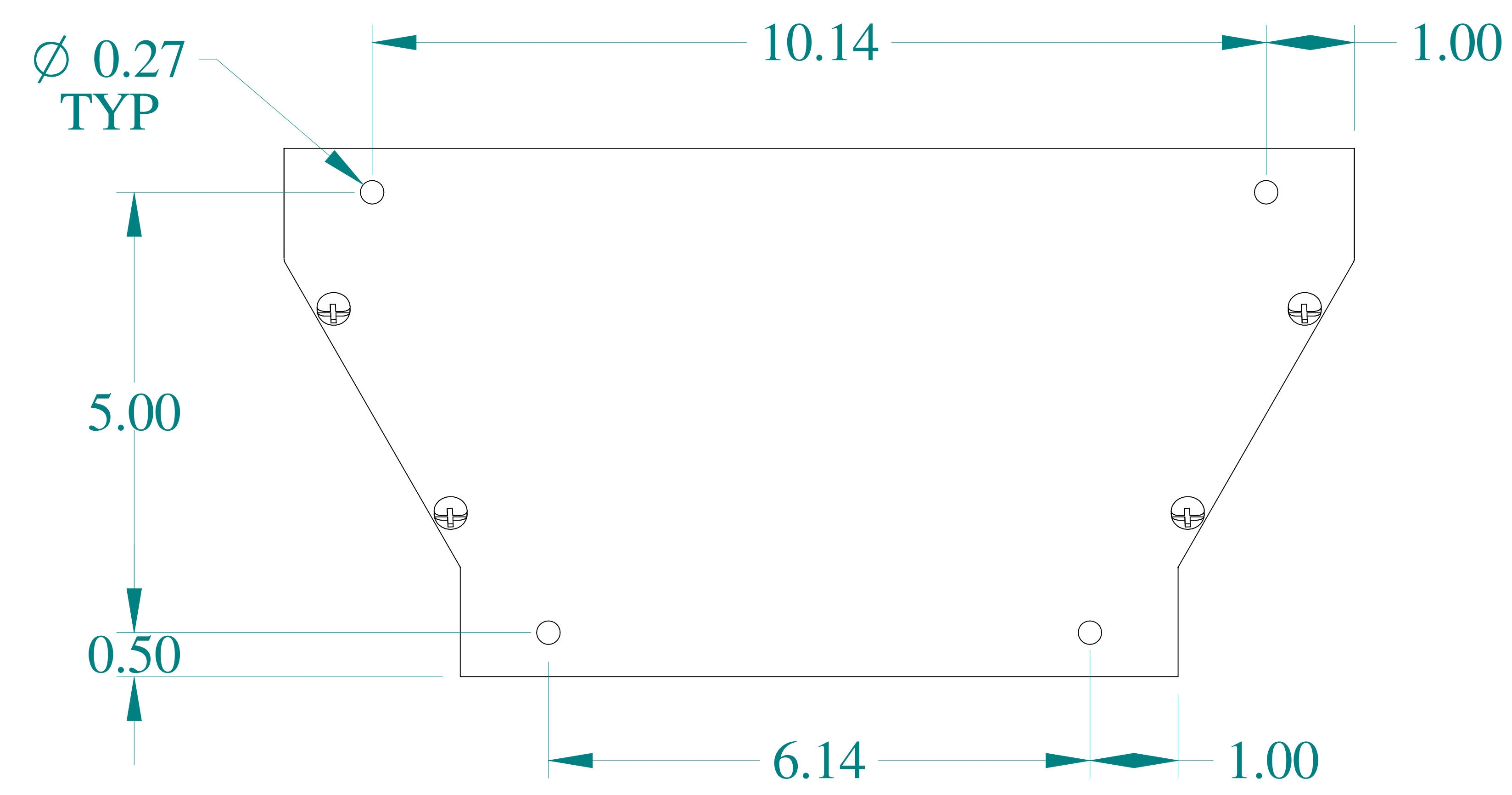
TOP VIEW
