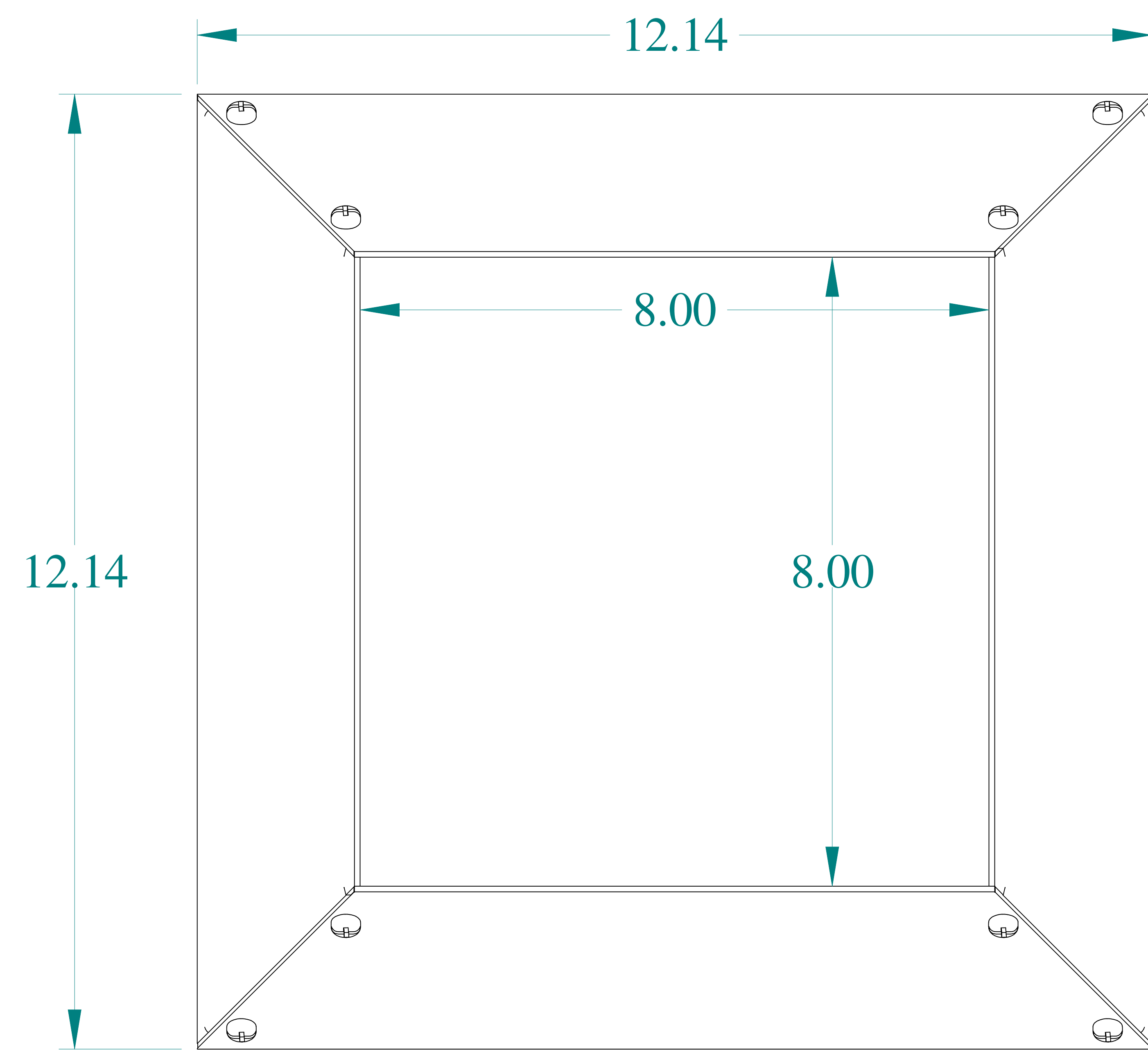
FRONT VIEW
