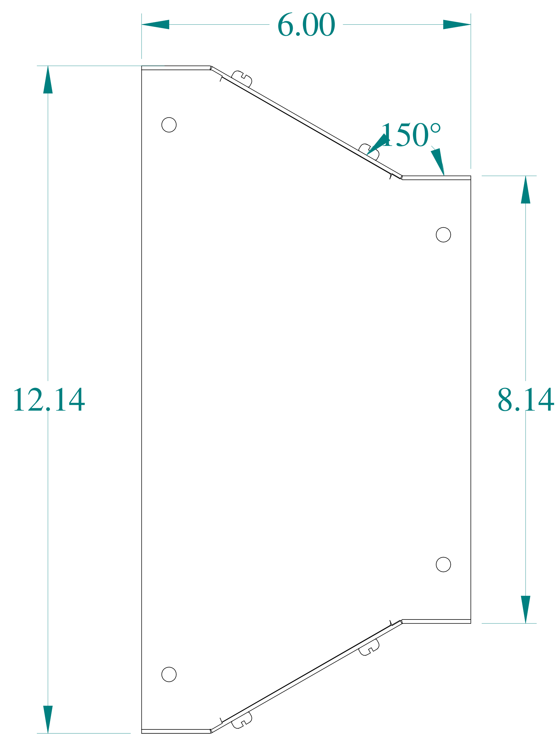
SIDE VIEW
