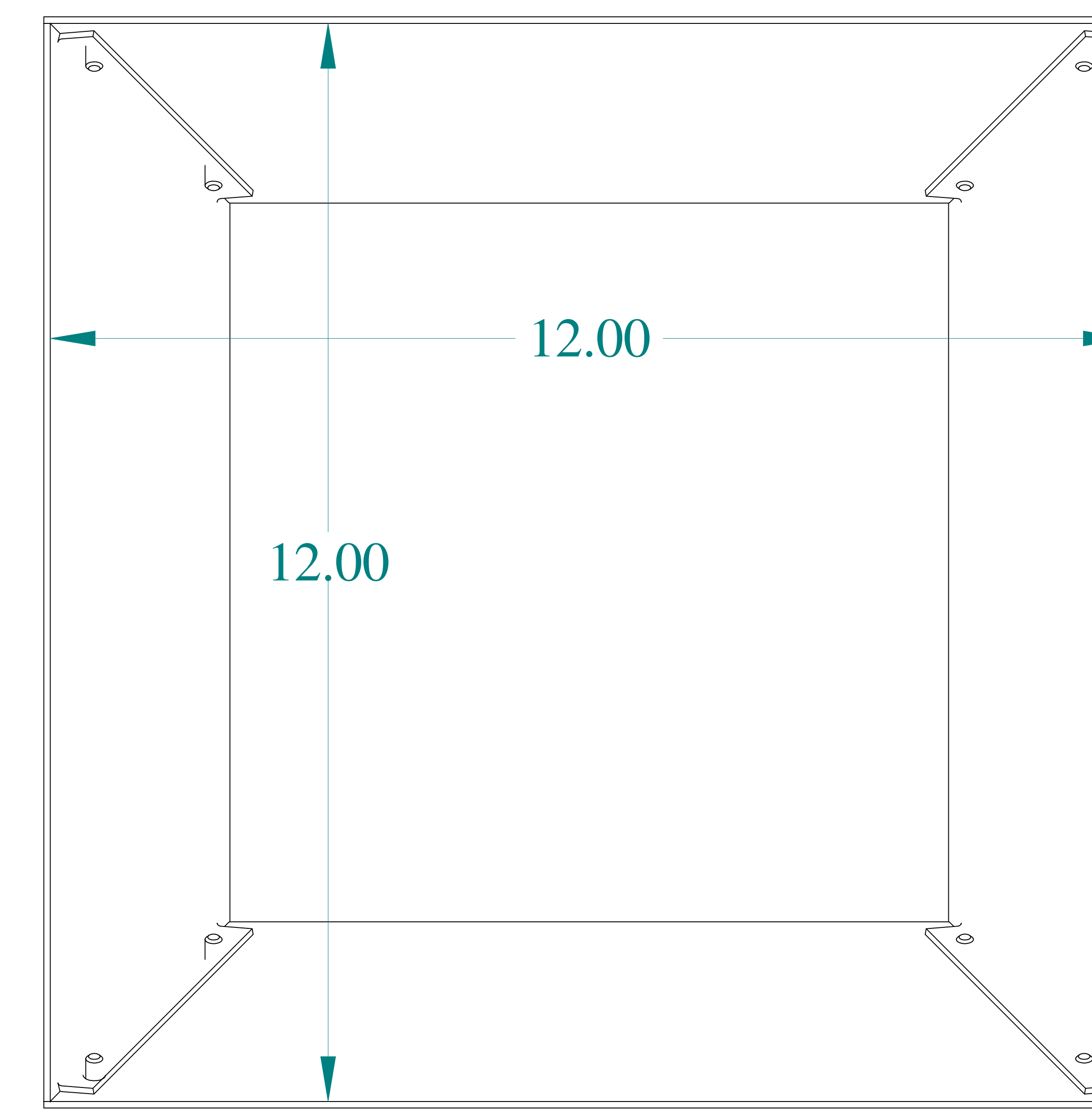
BACK VIEW
