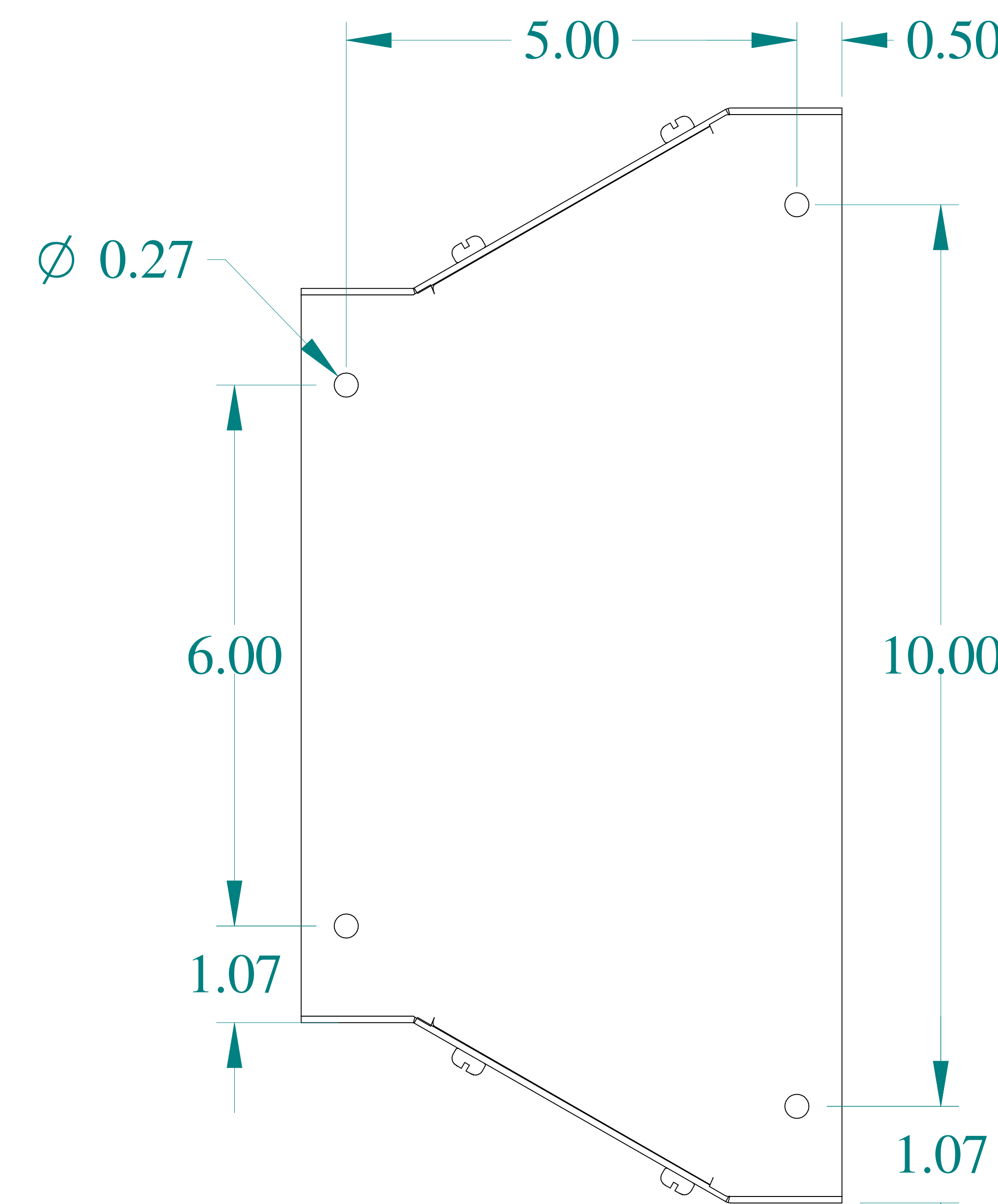
SIDE VIEW
