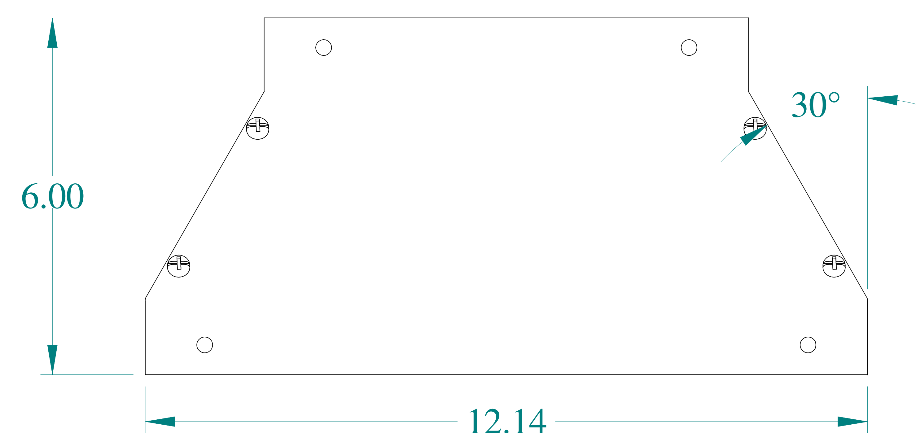
BOTTOM VIEW
