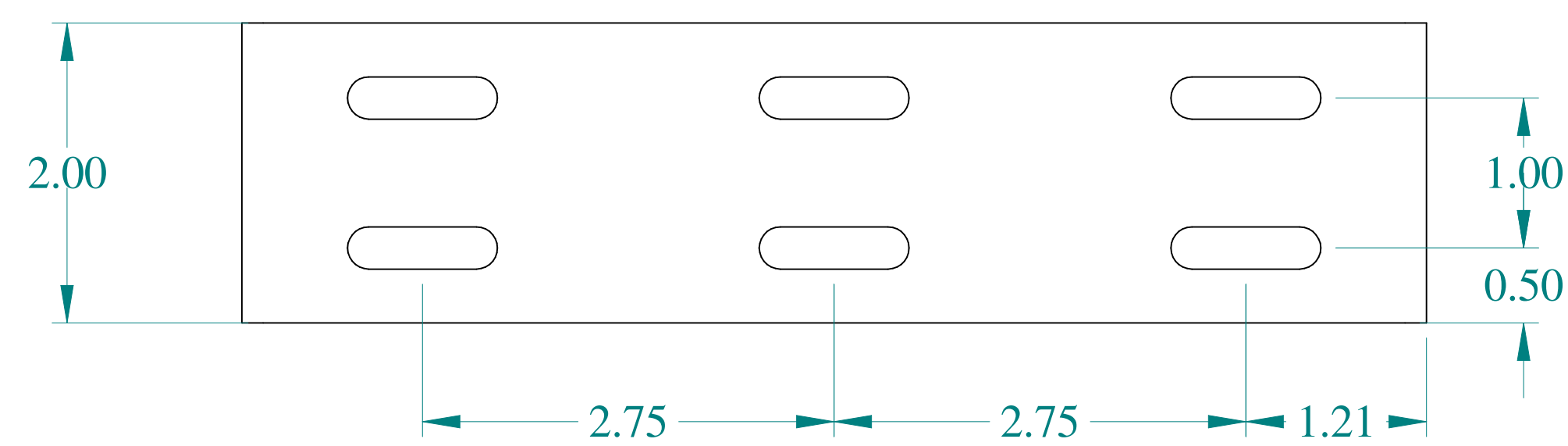
BOTTOM VIEW
