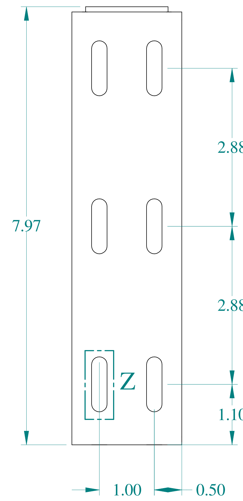
SIDE VIEW
