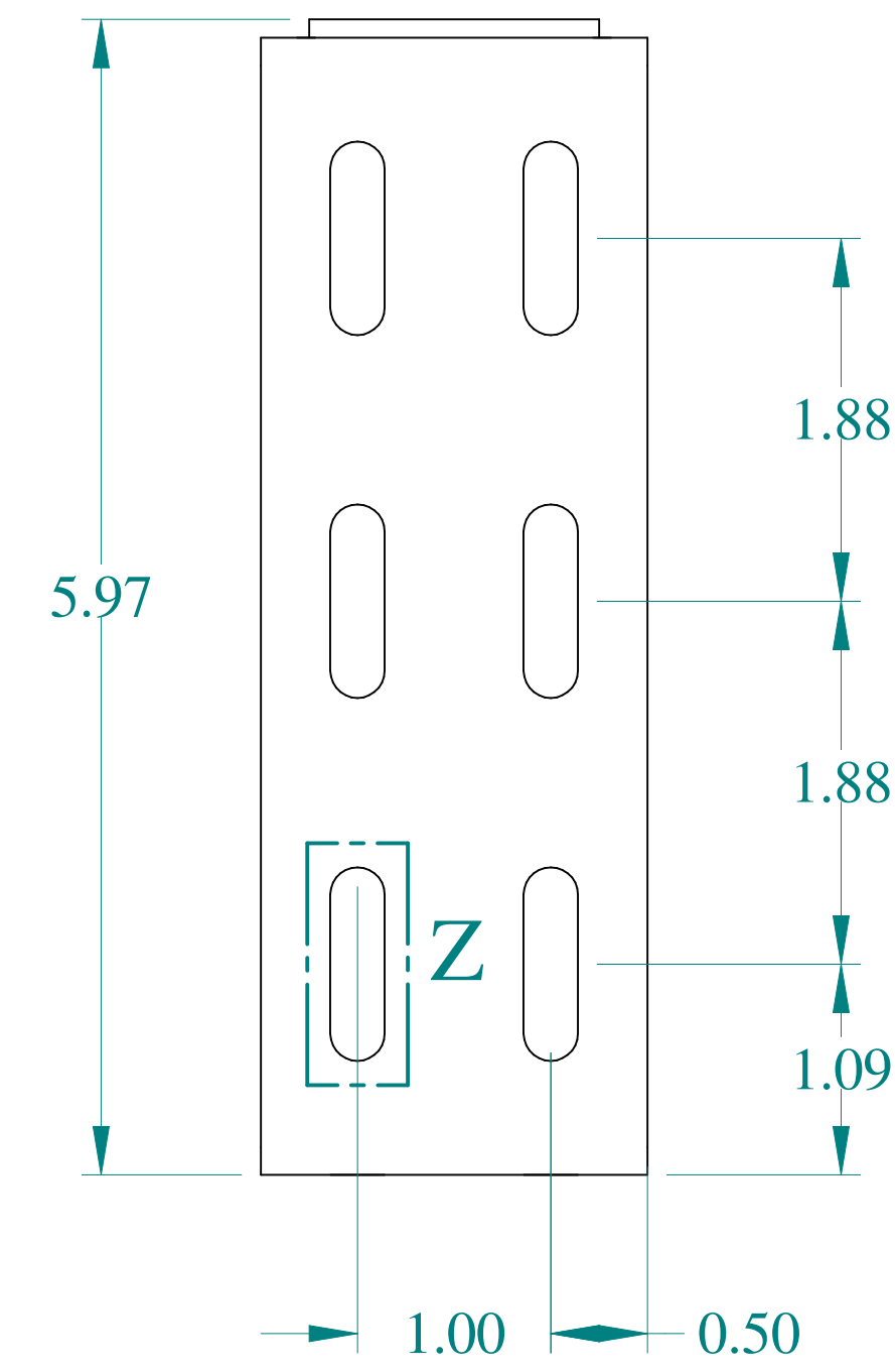
SIDE VIEW
