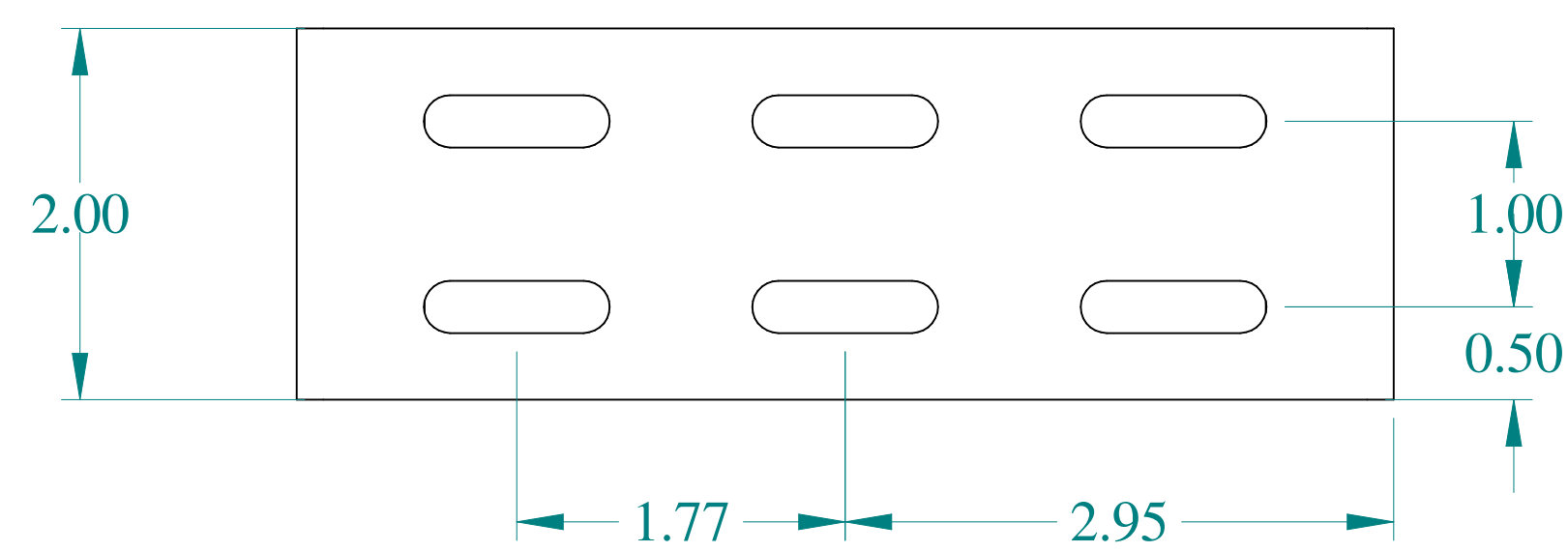
BOTTOM VIEW
