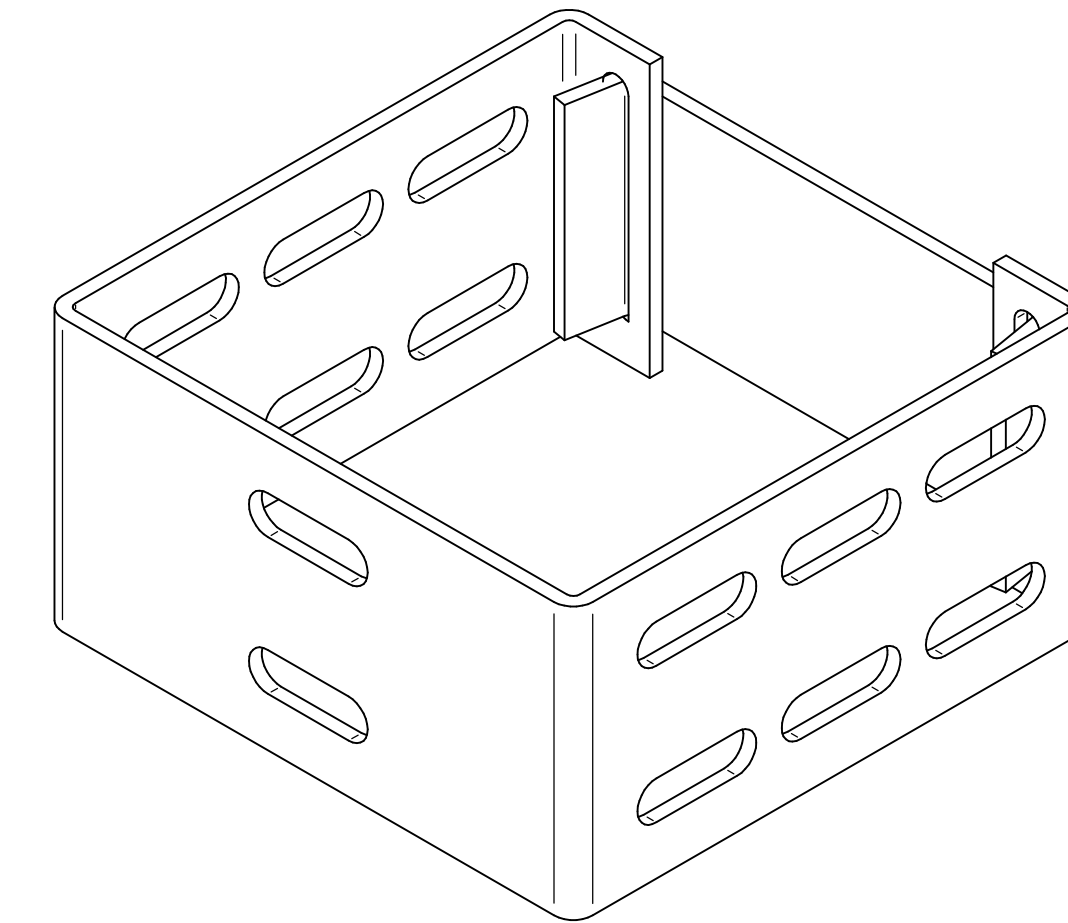
ISOMETRIC VIEWS
