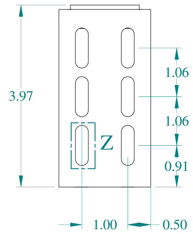
SIDE VIEW
