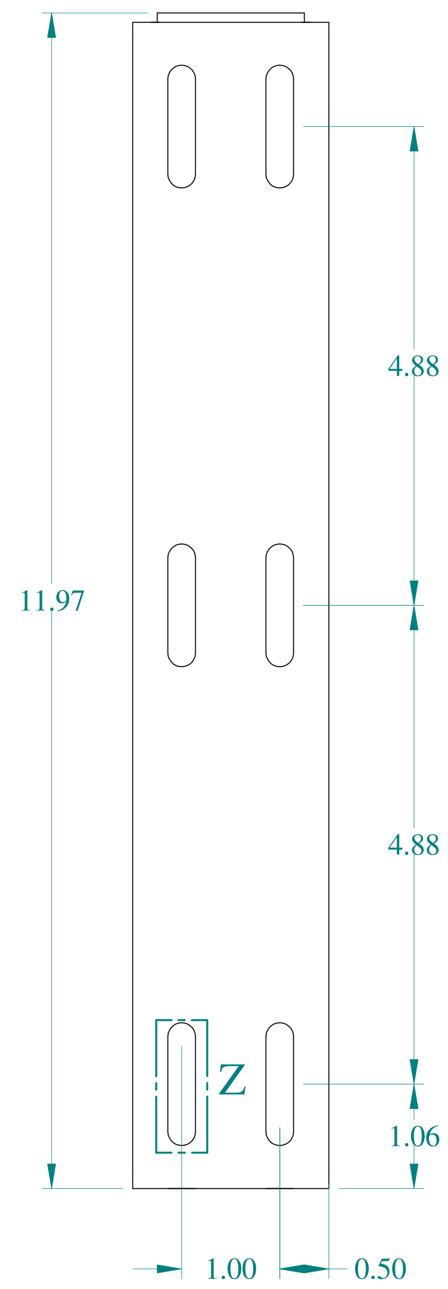
SIDE VIEW
