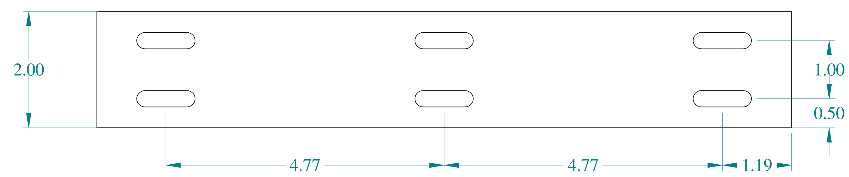
BOTTOM VIEW
