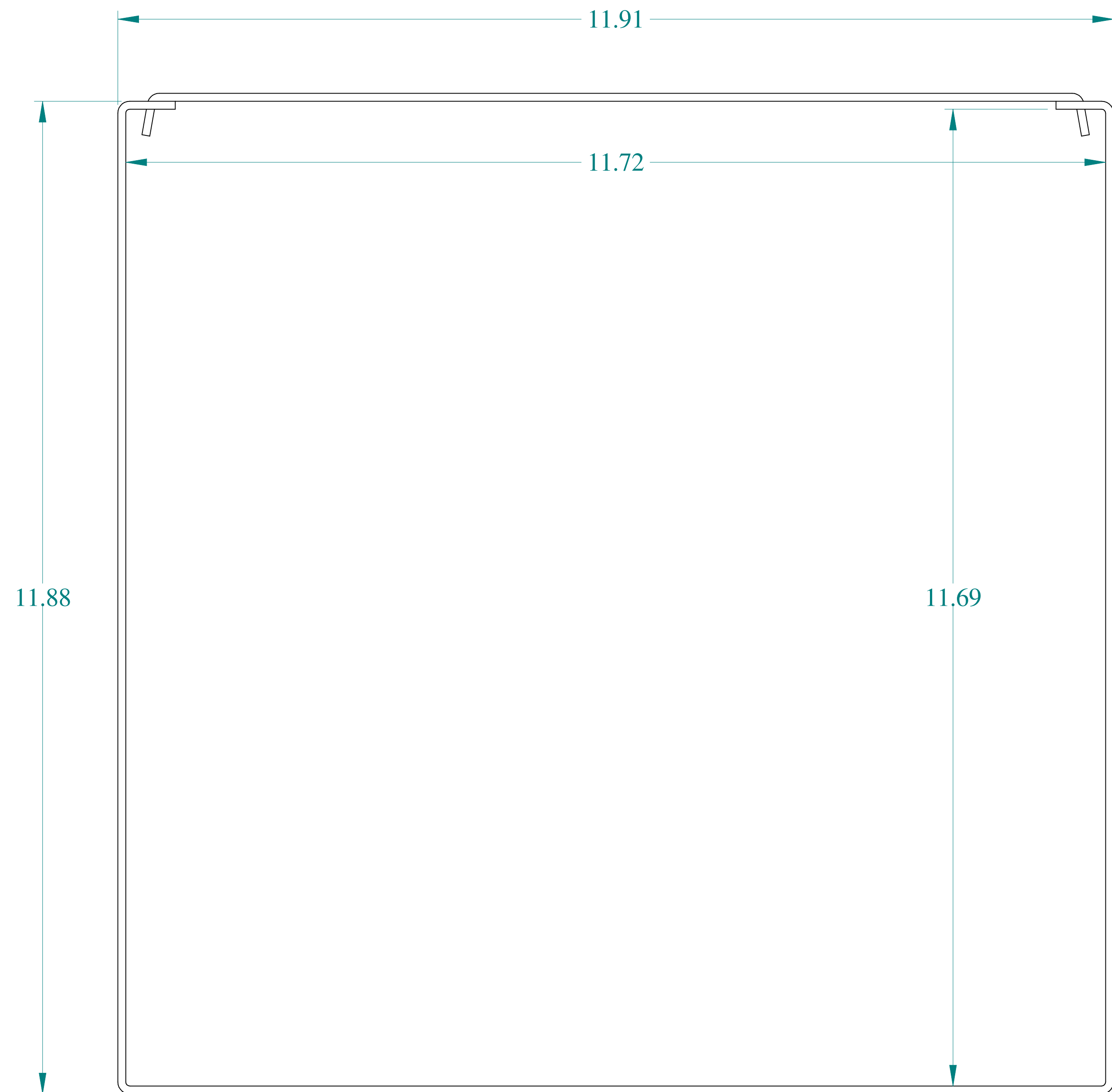
FRONT VIEW
