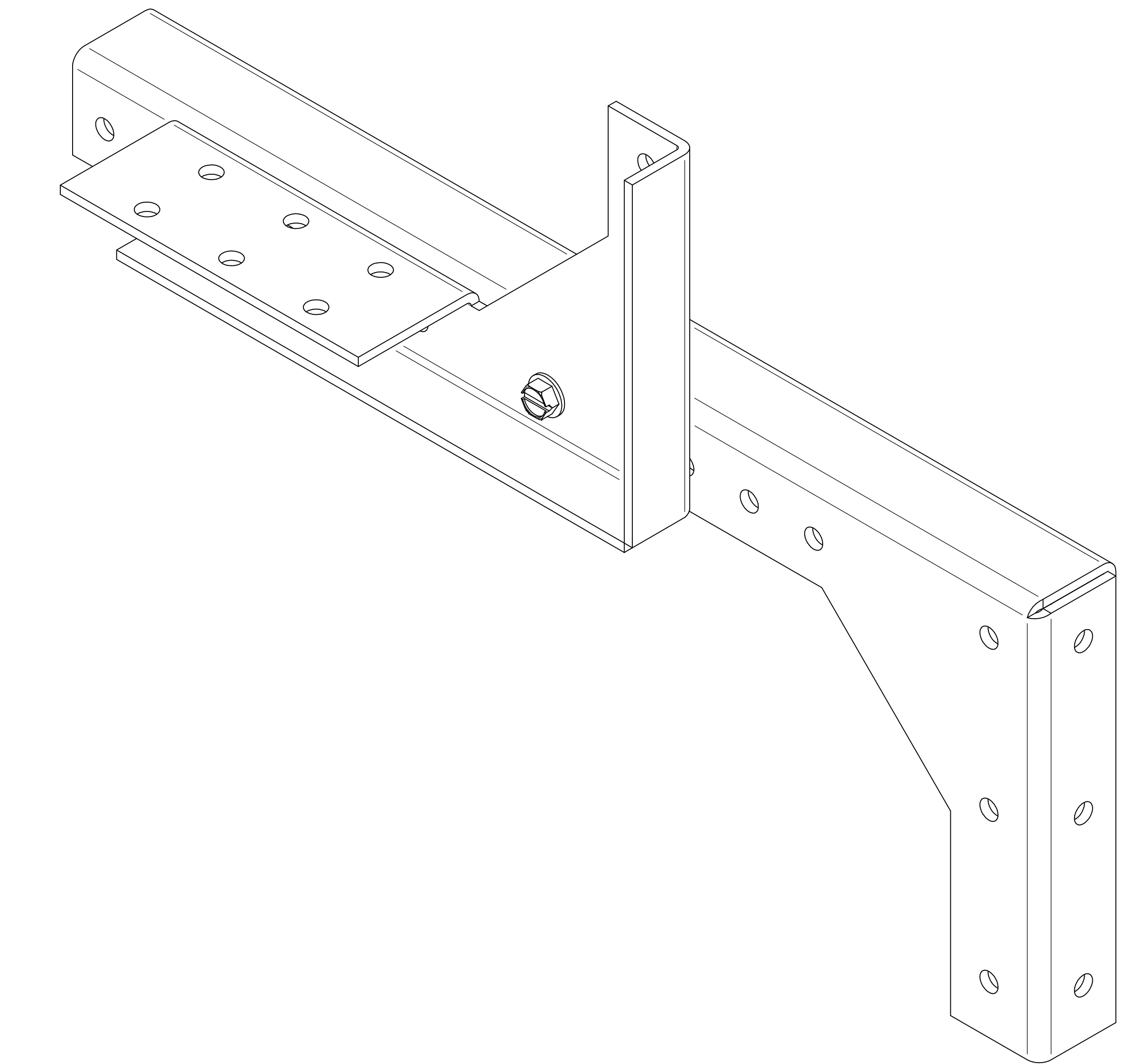
ISOMETRIC VIEWS
