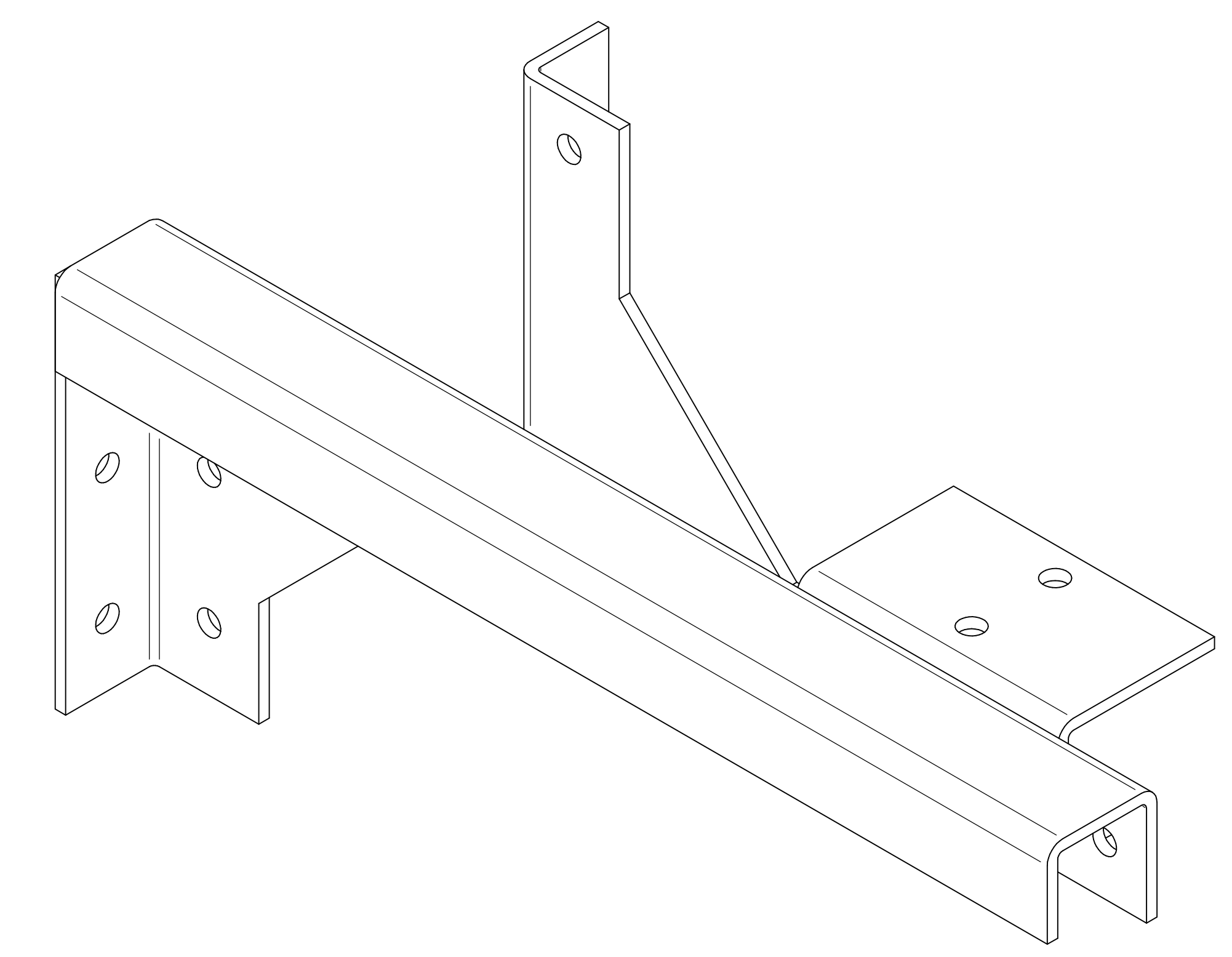
ISOMETRIC VIEWS
