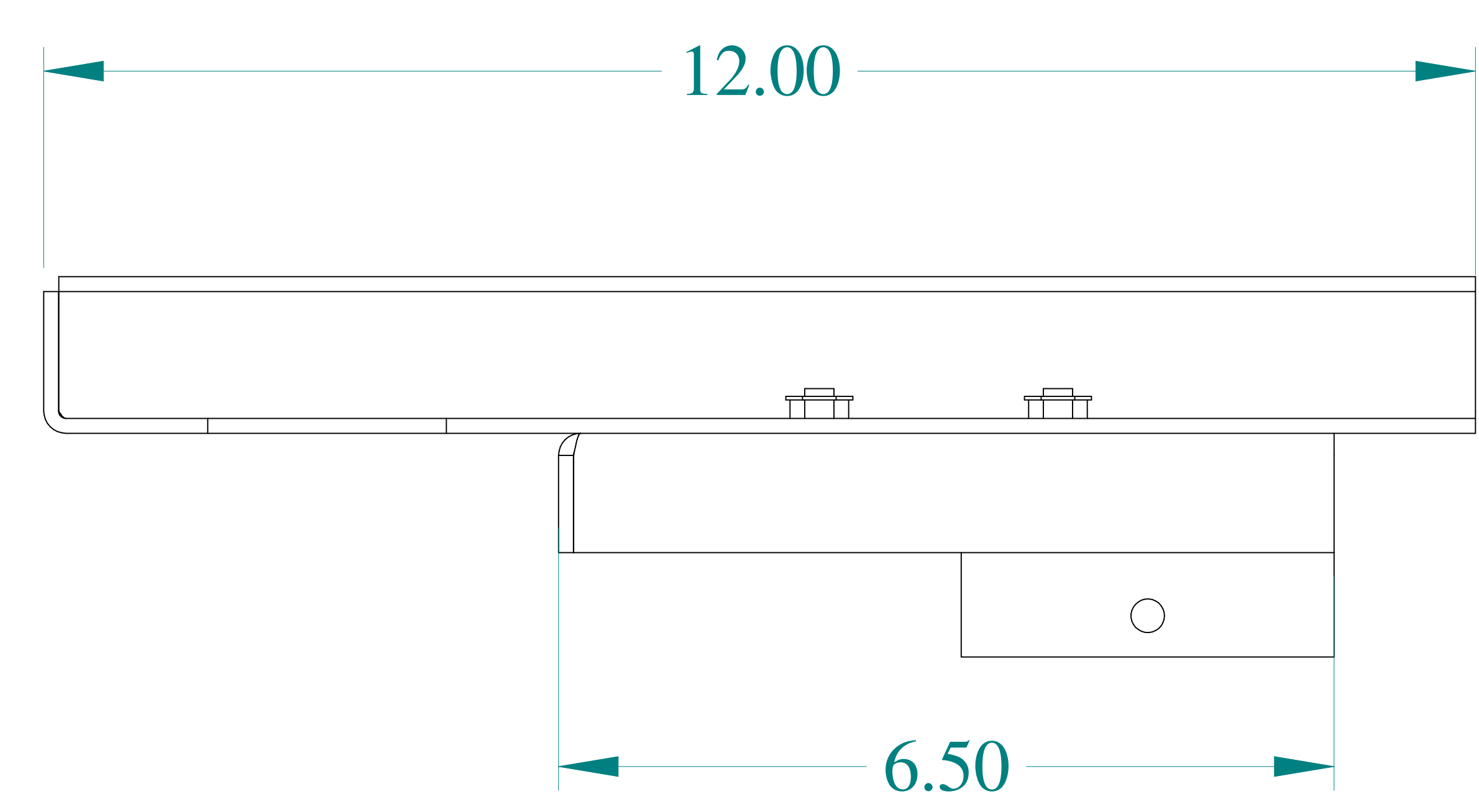
BOTTOM VIEW
