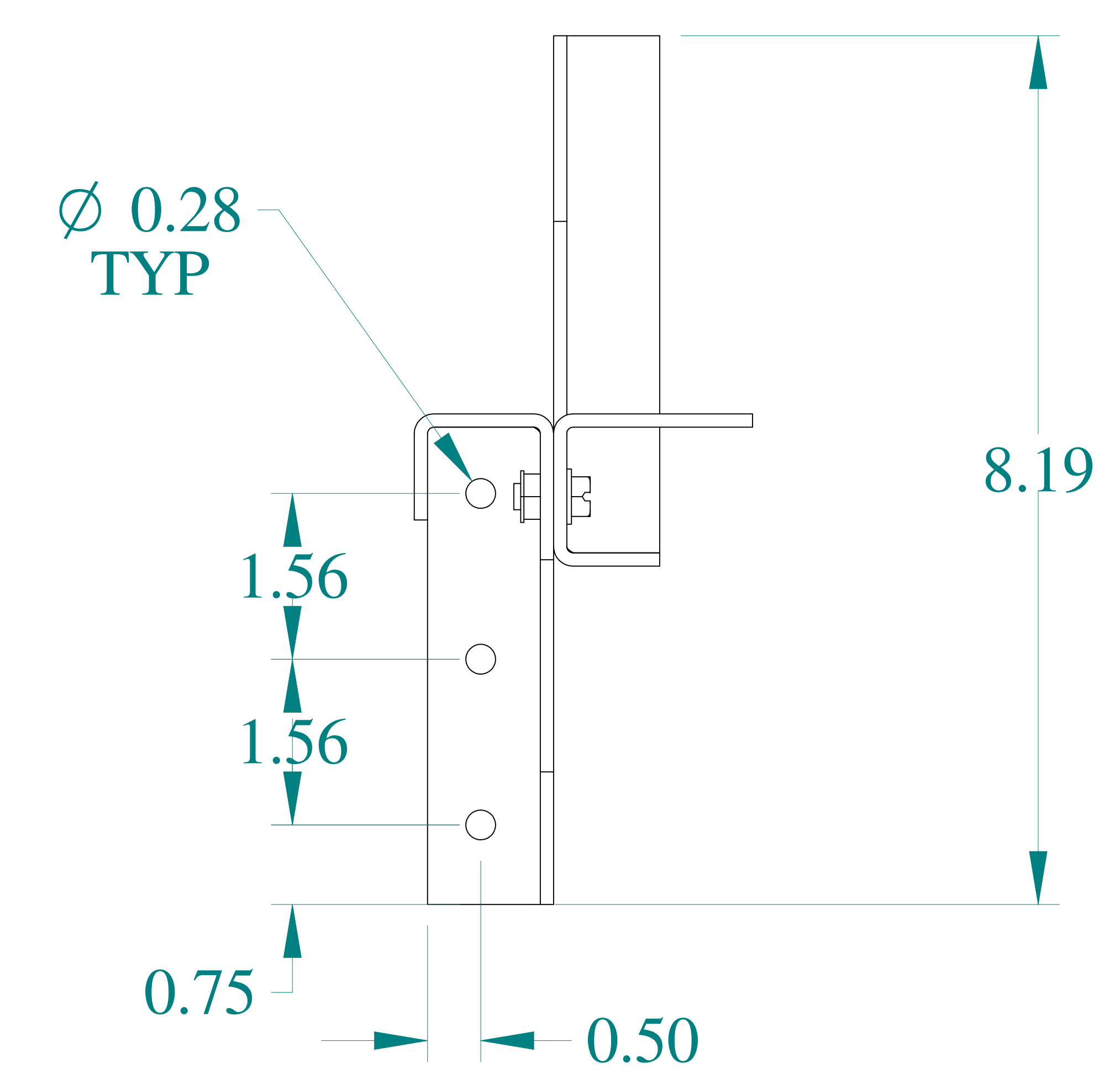
SIDE VIEW
