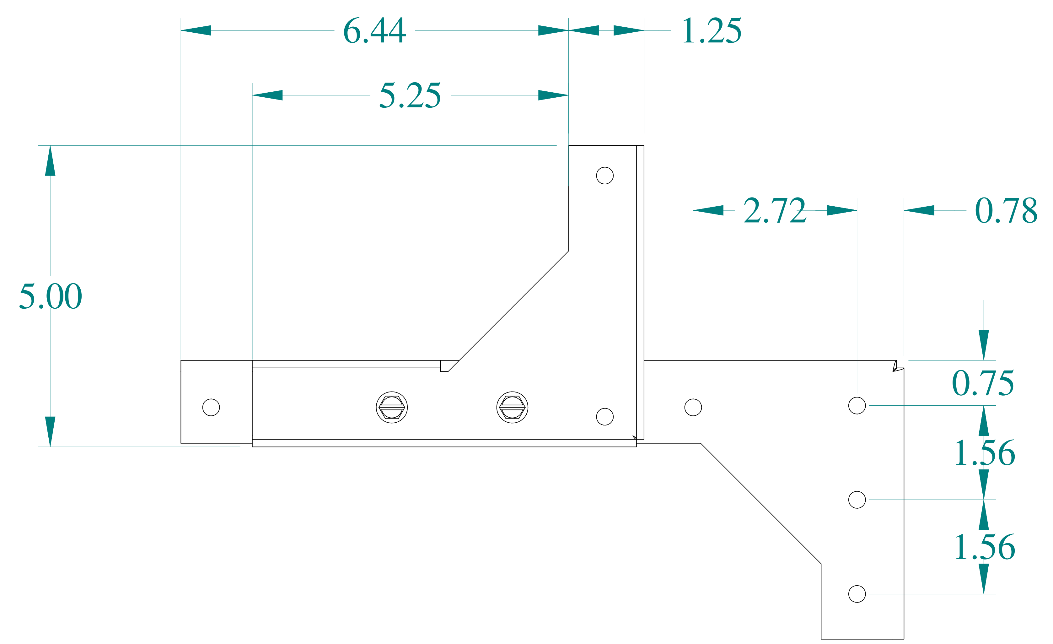
BACK VIEW
