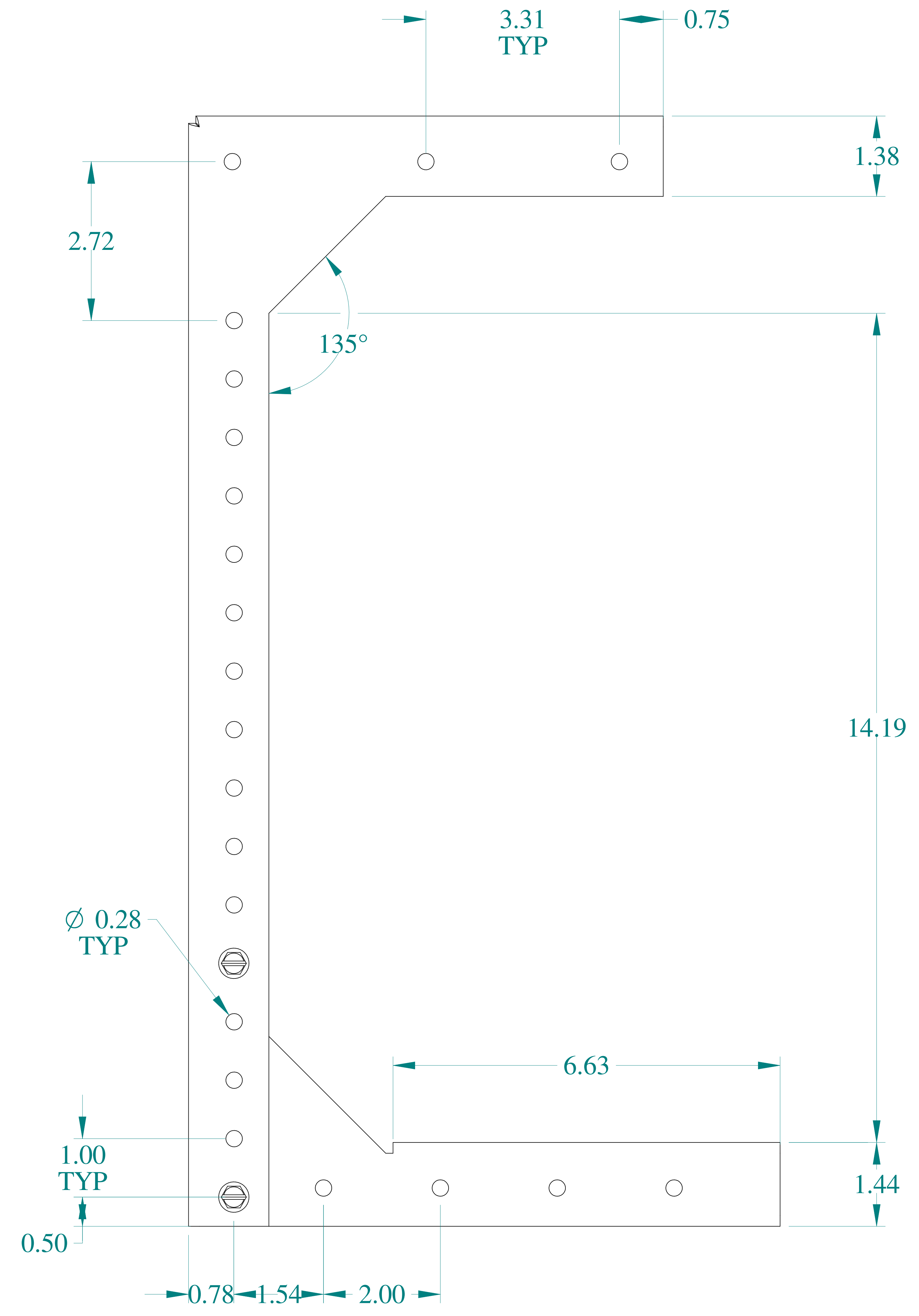
FRONT VIEW
