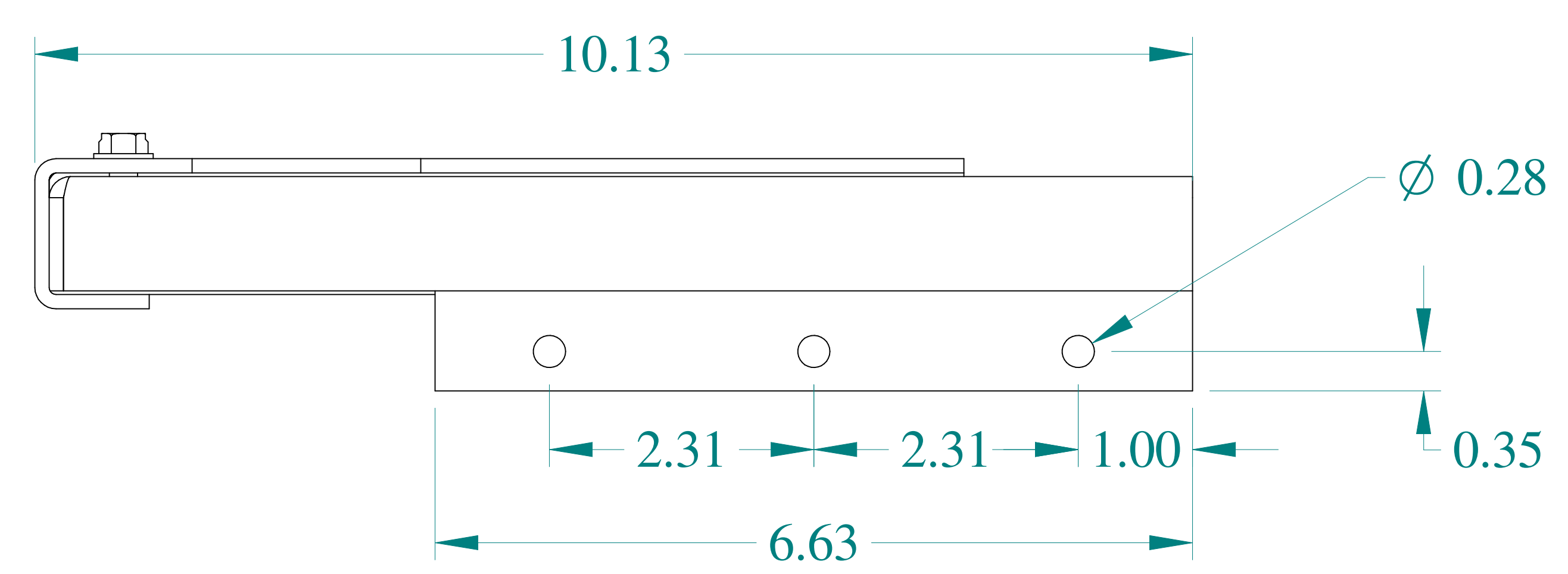
BOTTOM VIEW
