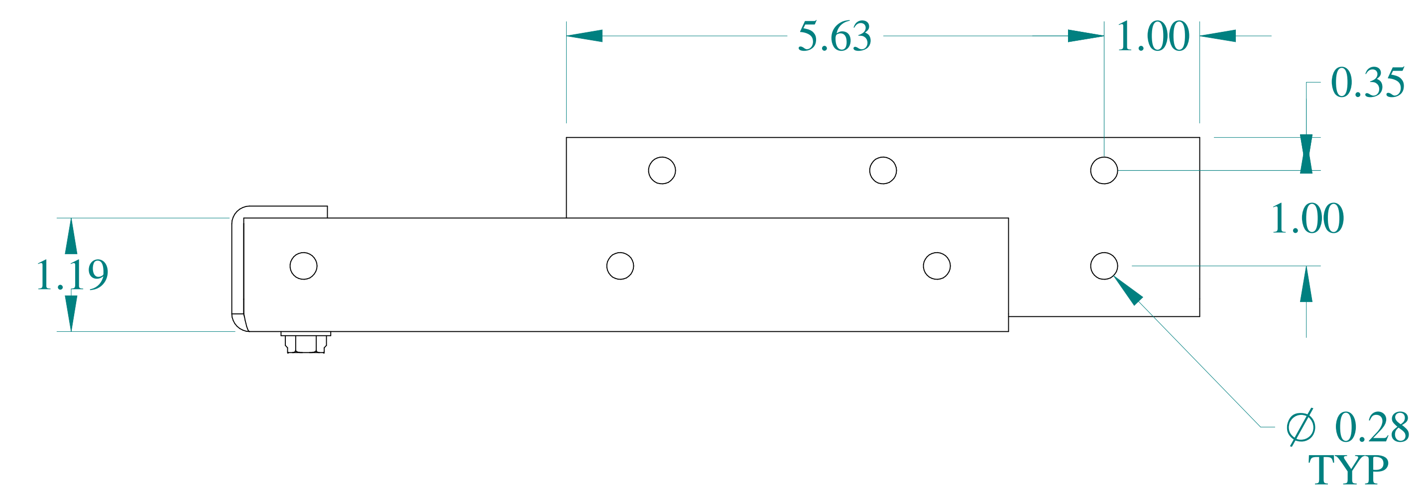
TOP VIEW
