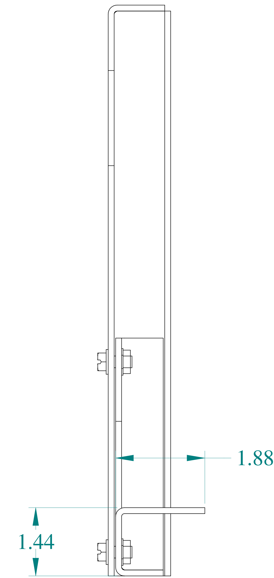
SIDE VIEW
