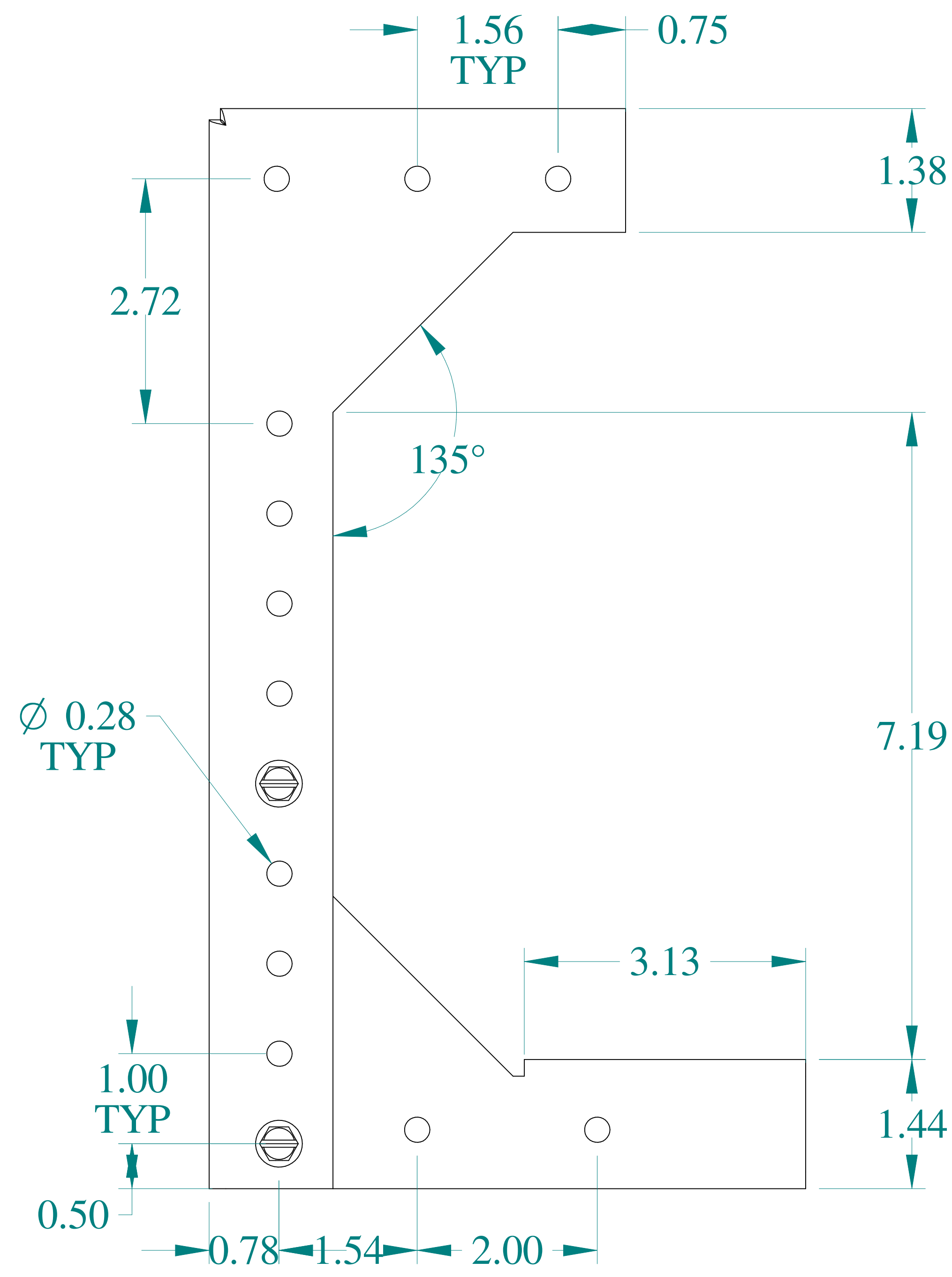
FRONT VIEW
