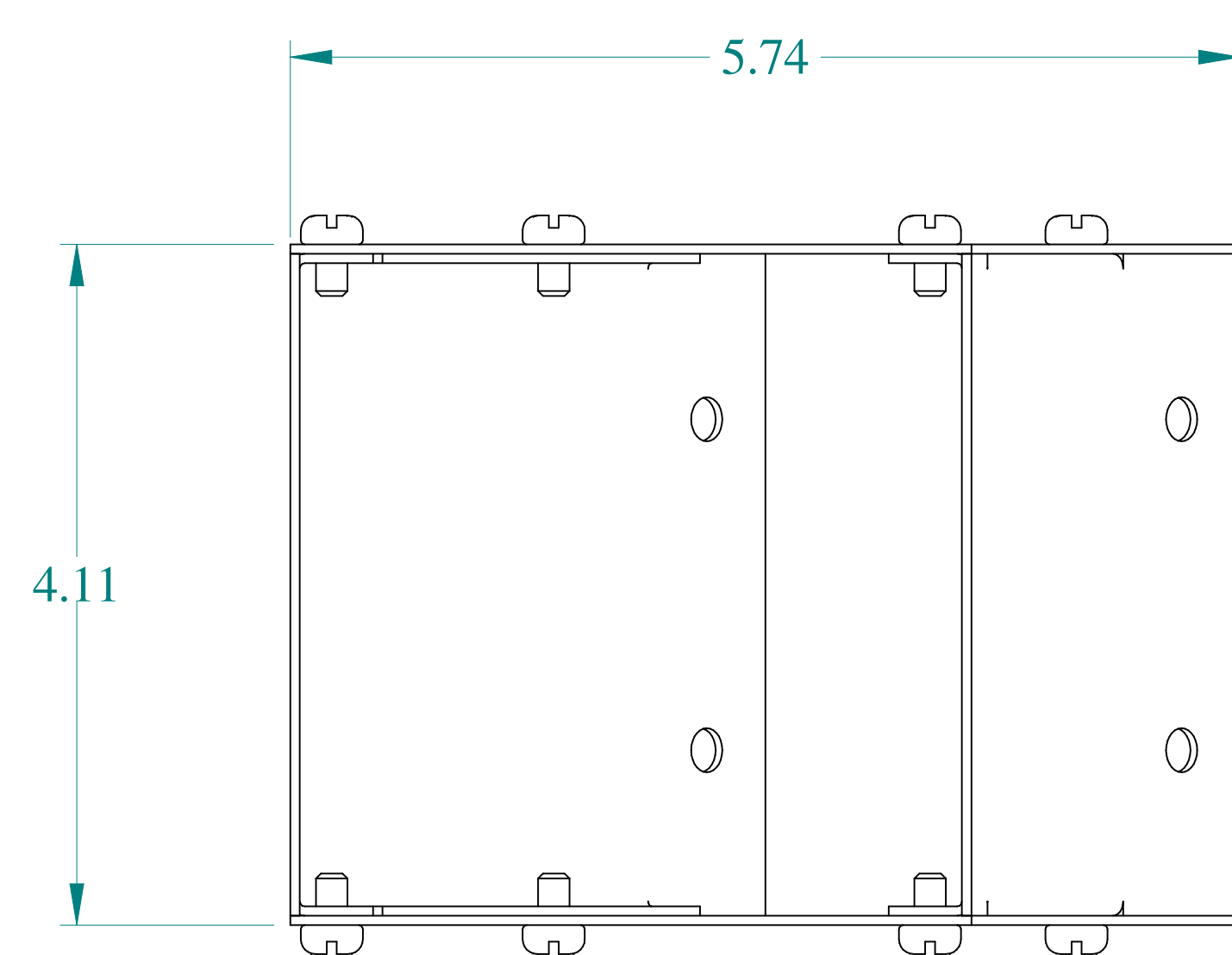
FRONT VIEW
