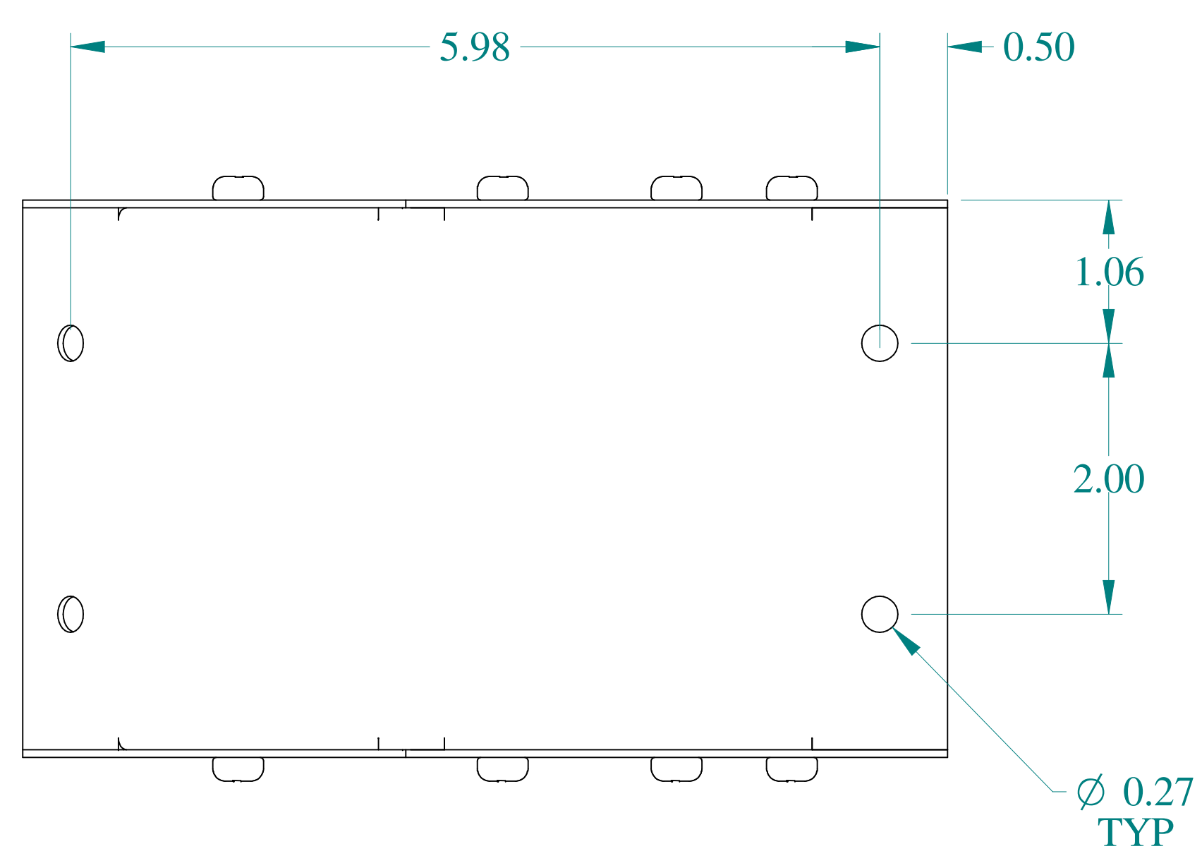
SIDE VIEW
