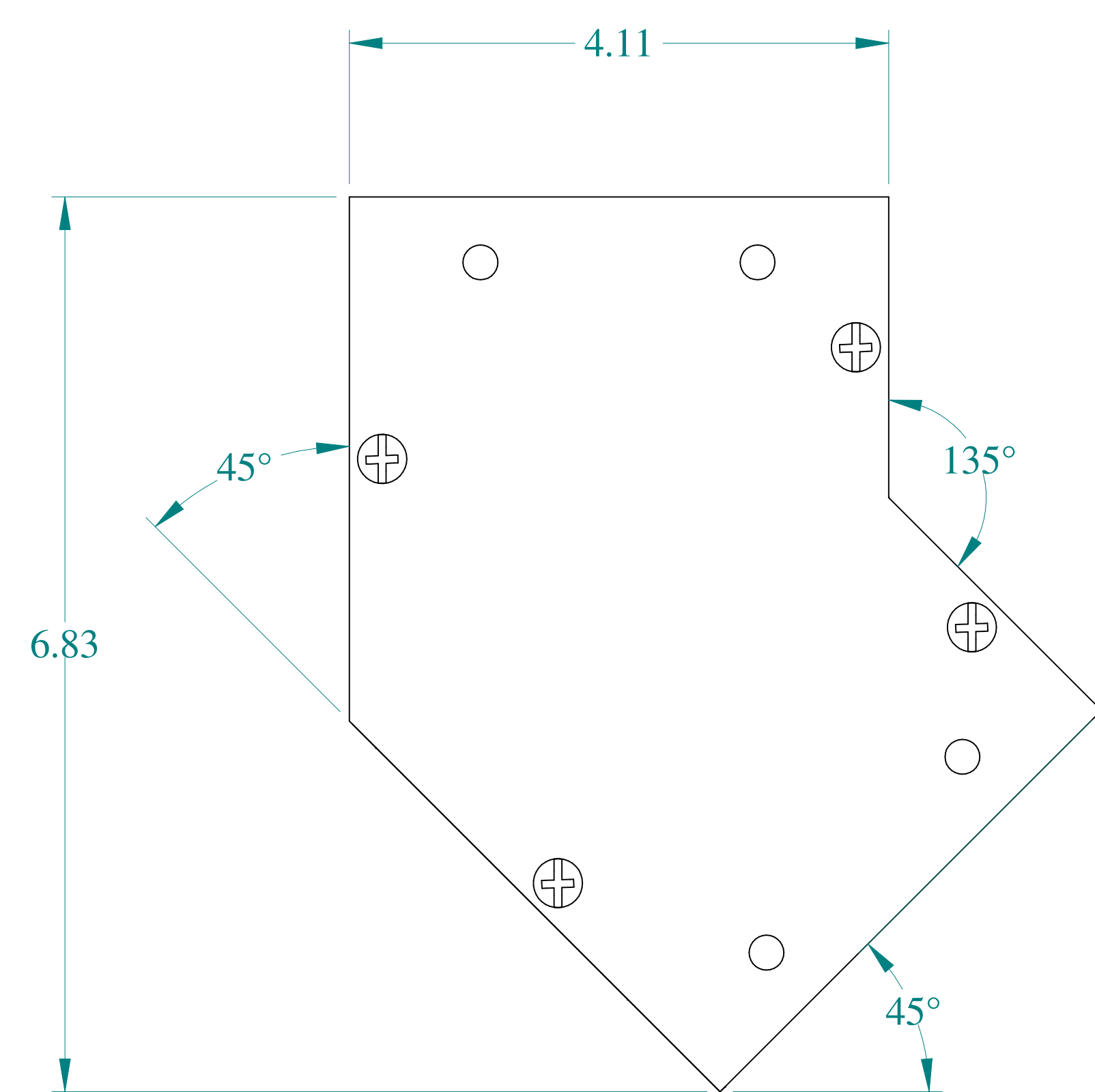
BOTTOM VIEW
