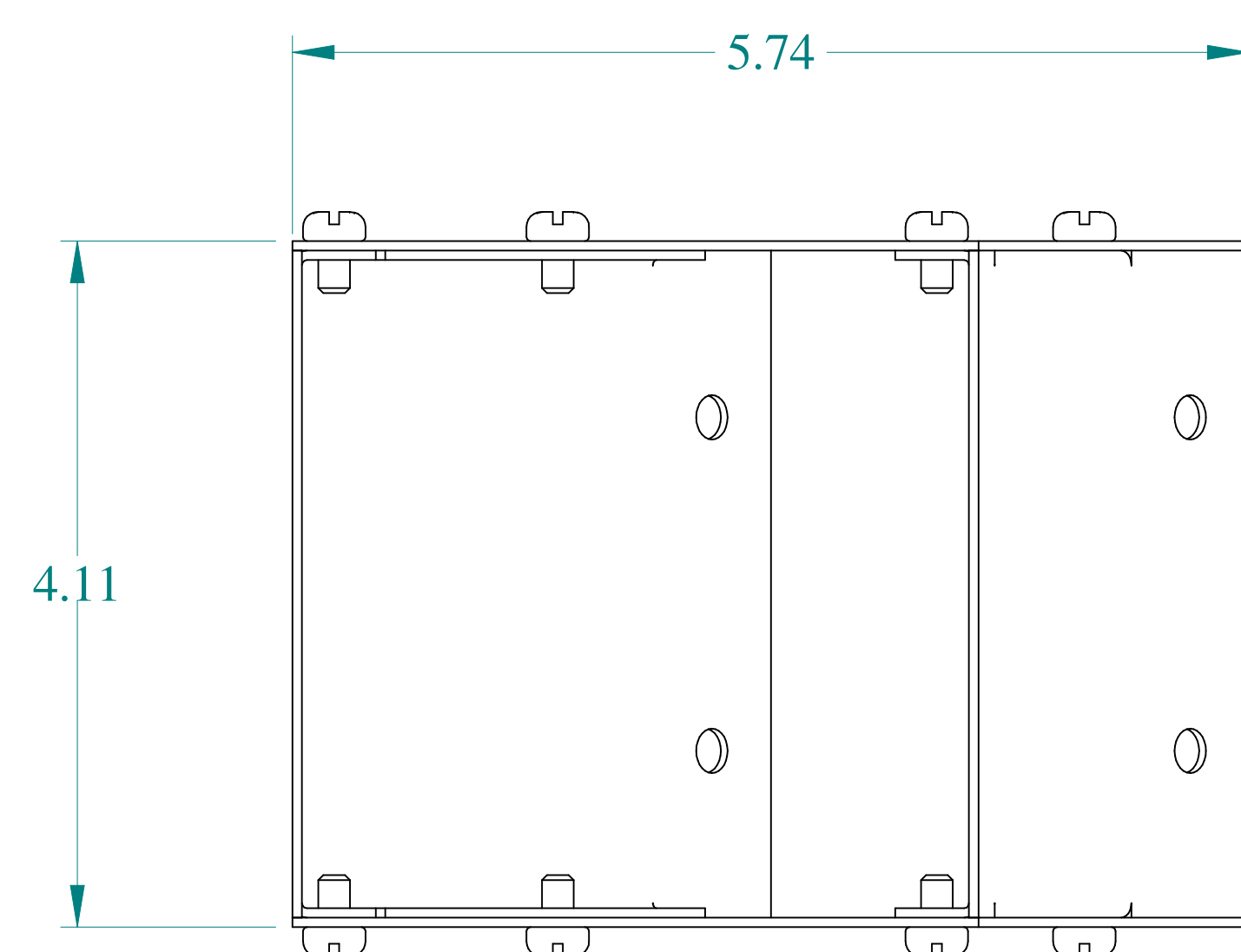
FRONT VIEW
