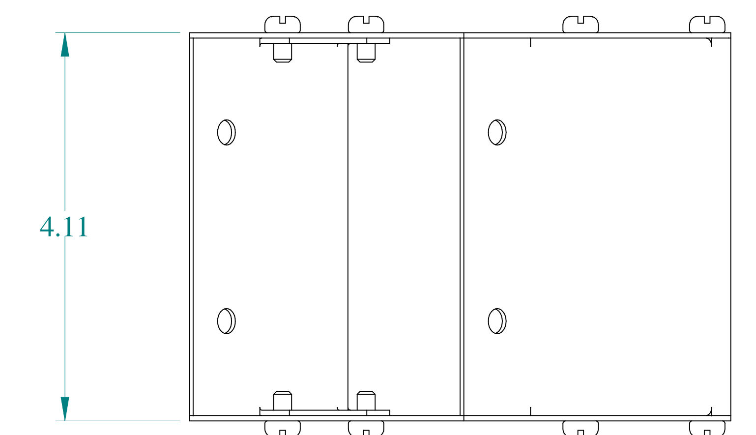
BACK VIEW
