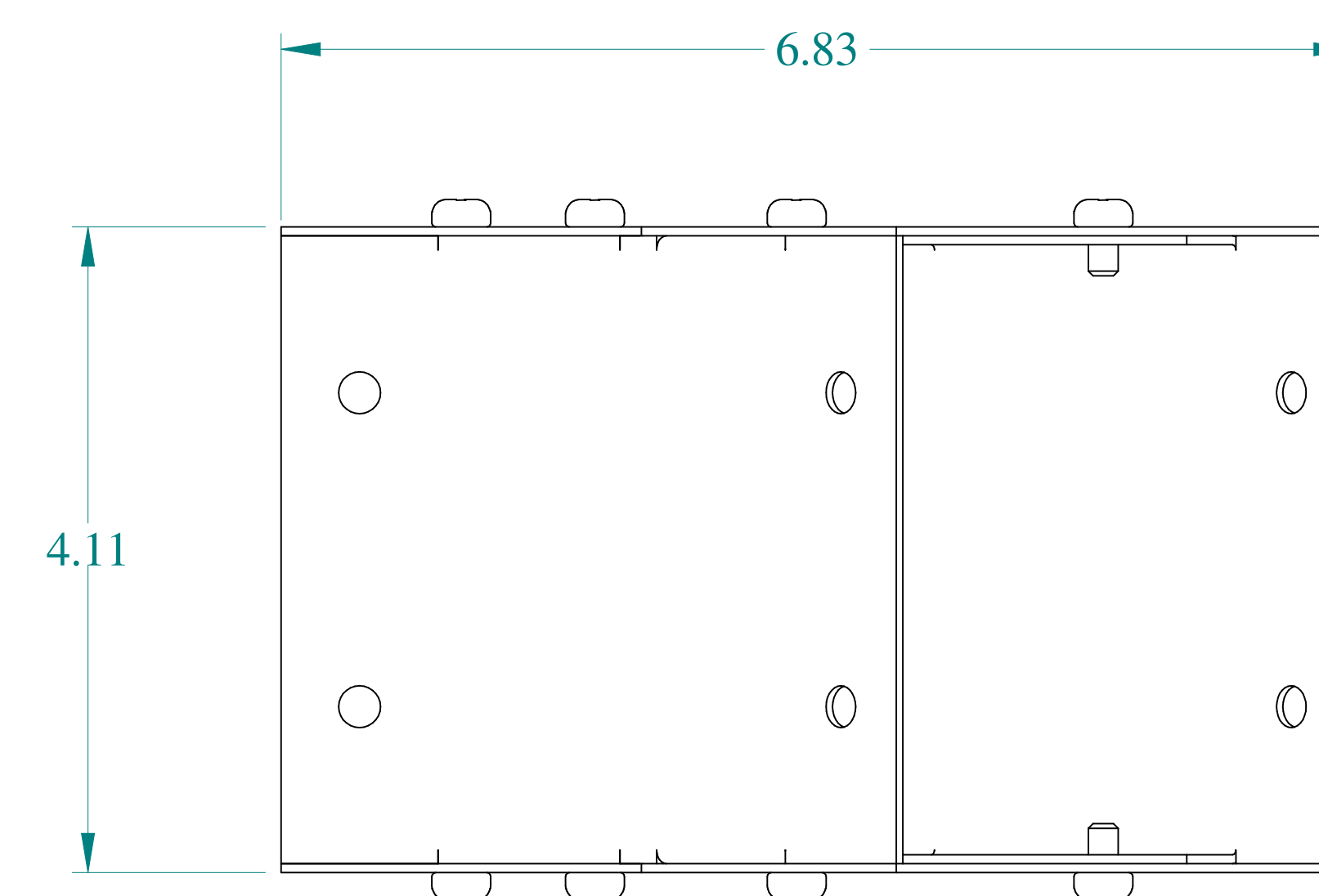
SIDE VIEW
