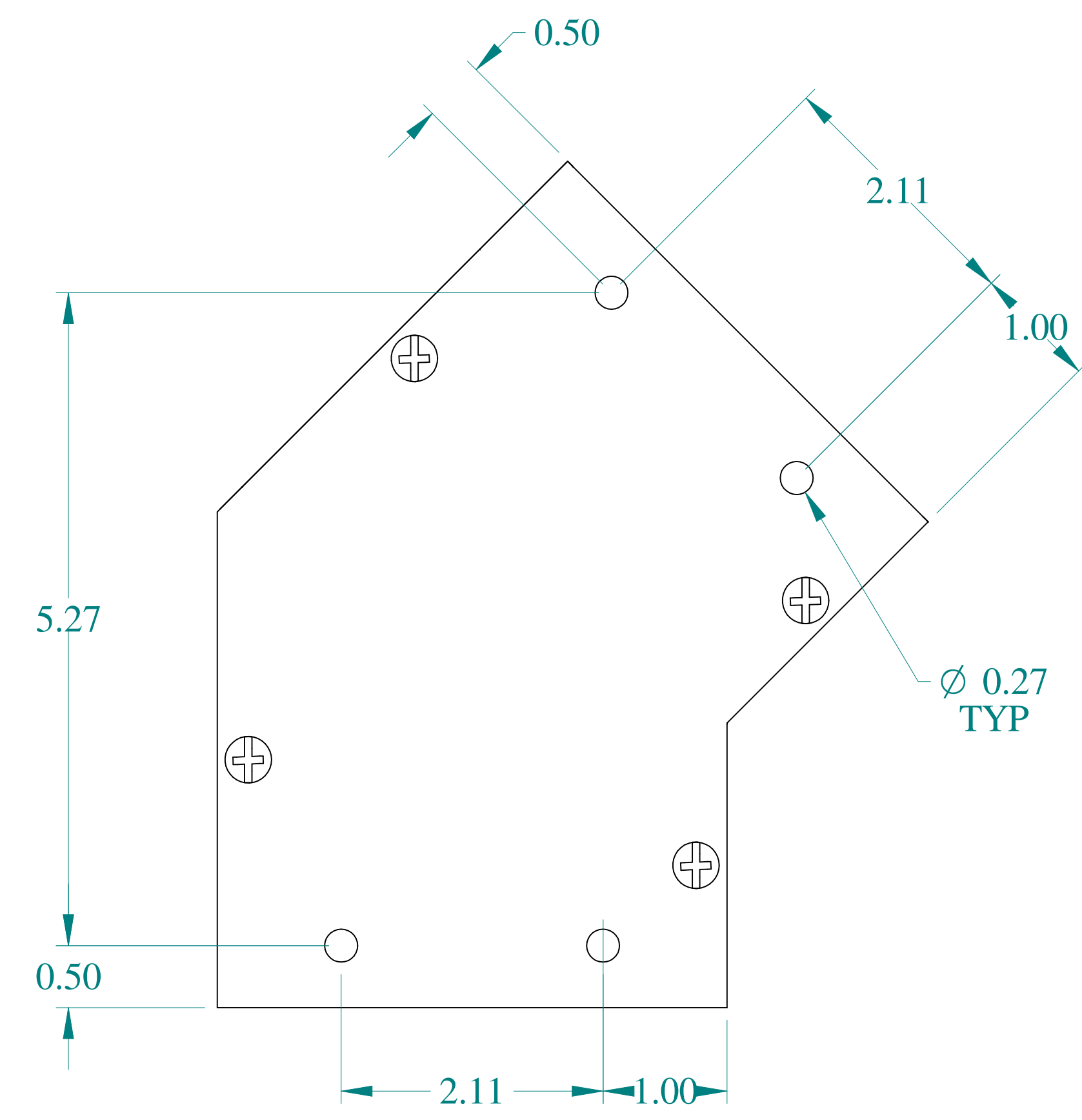
TOP VIEW
