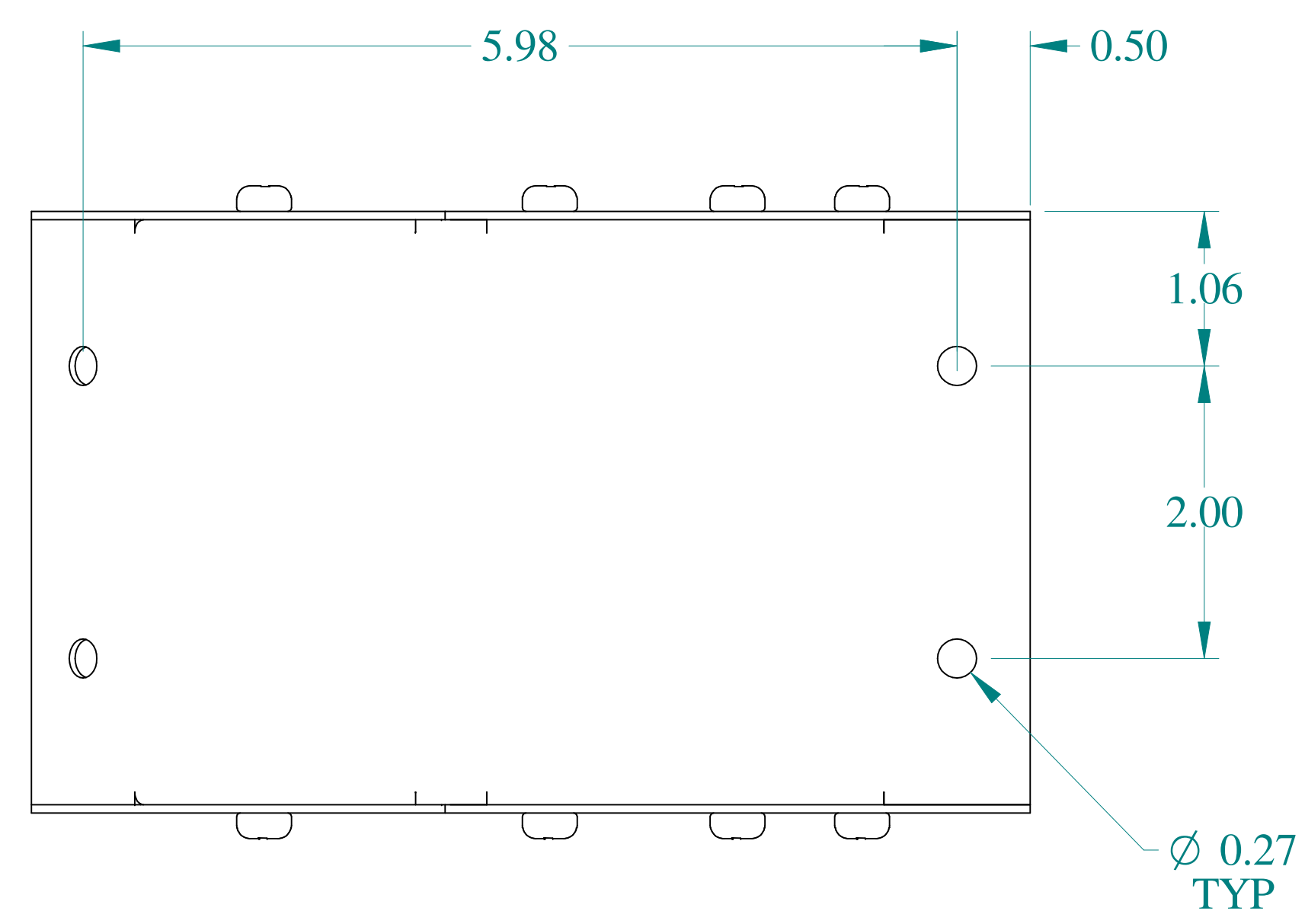
SIDE VIEW
