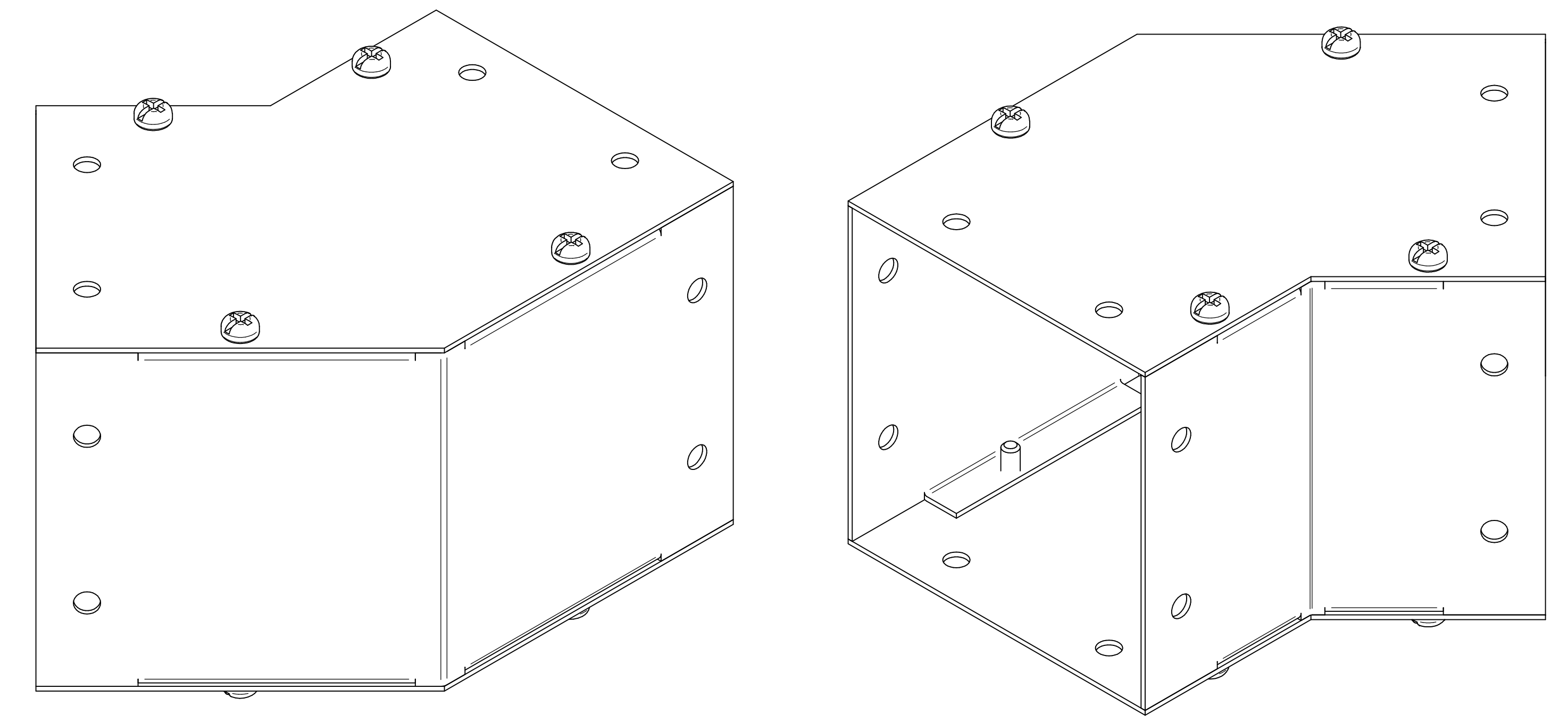
ISOMETRIC VIEWS
