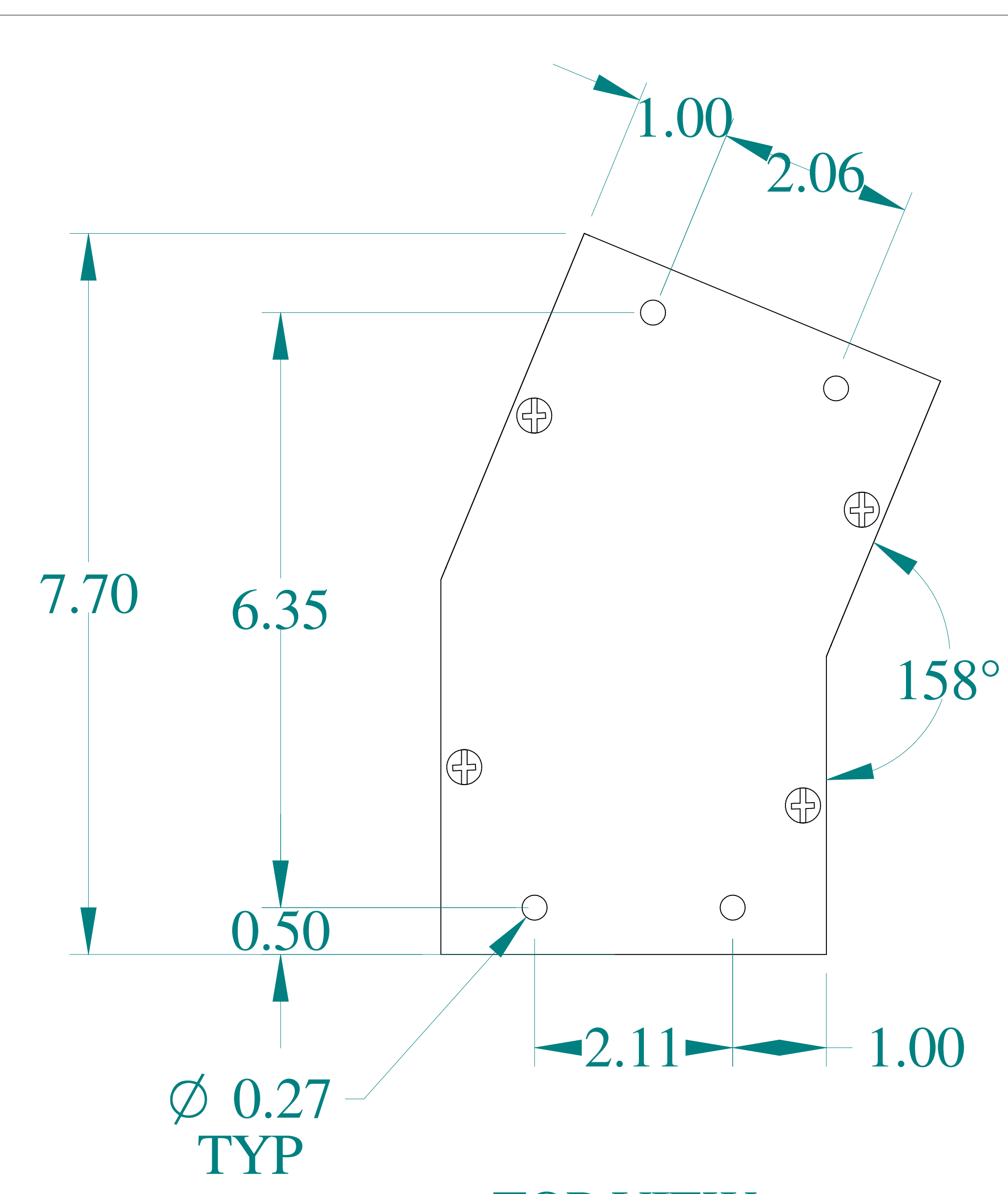
TOP VIEW
