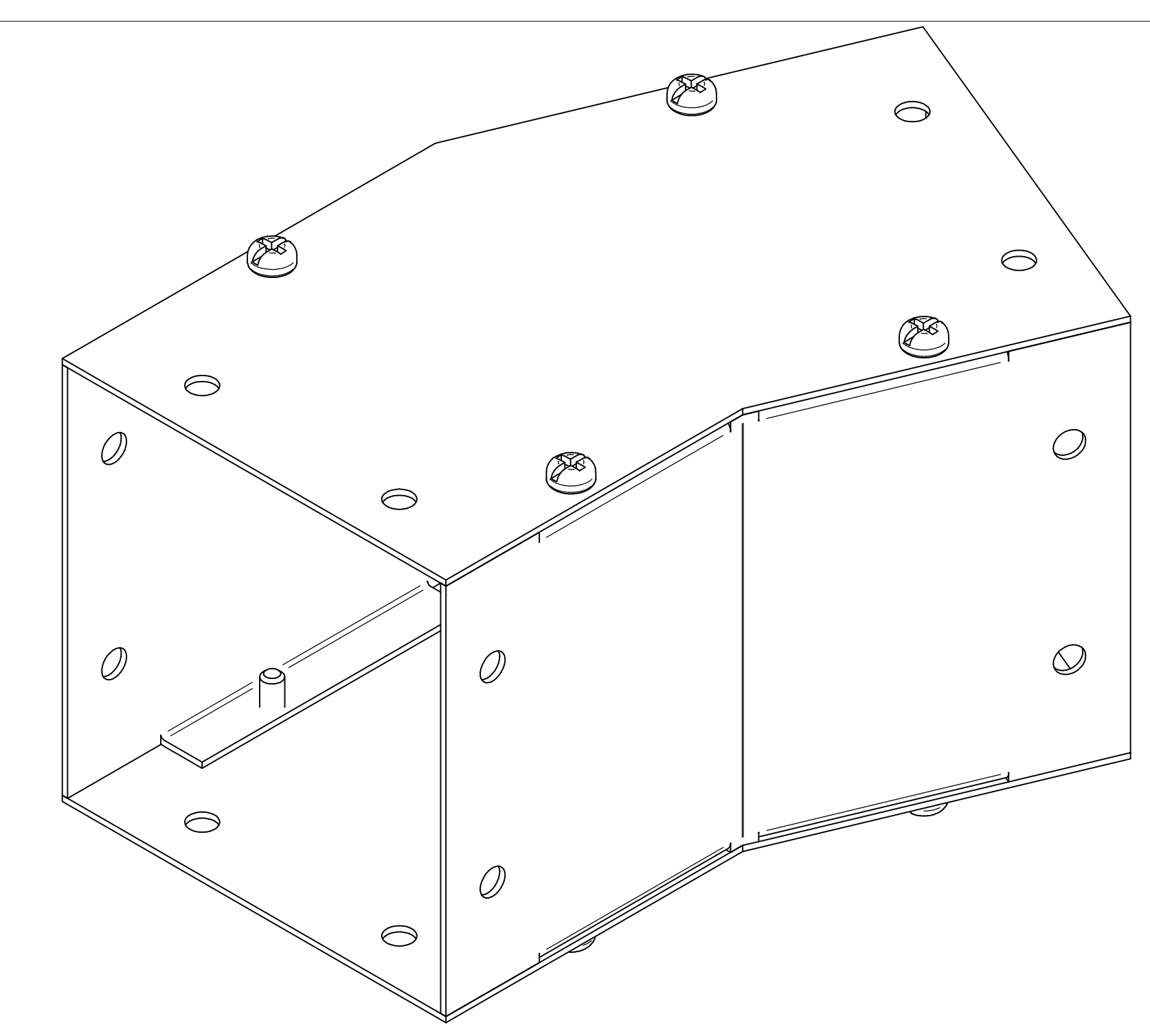
ISOMETRIC VIEWS
