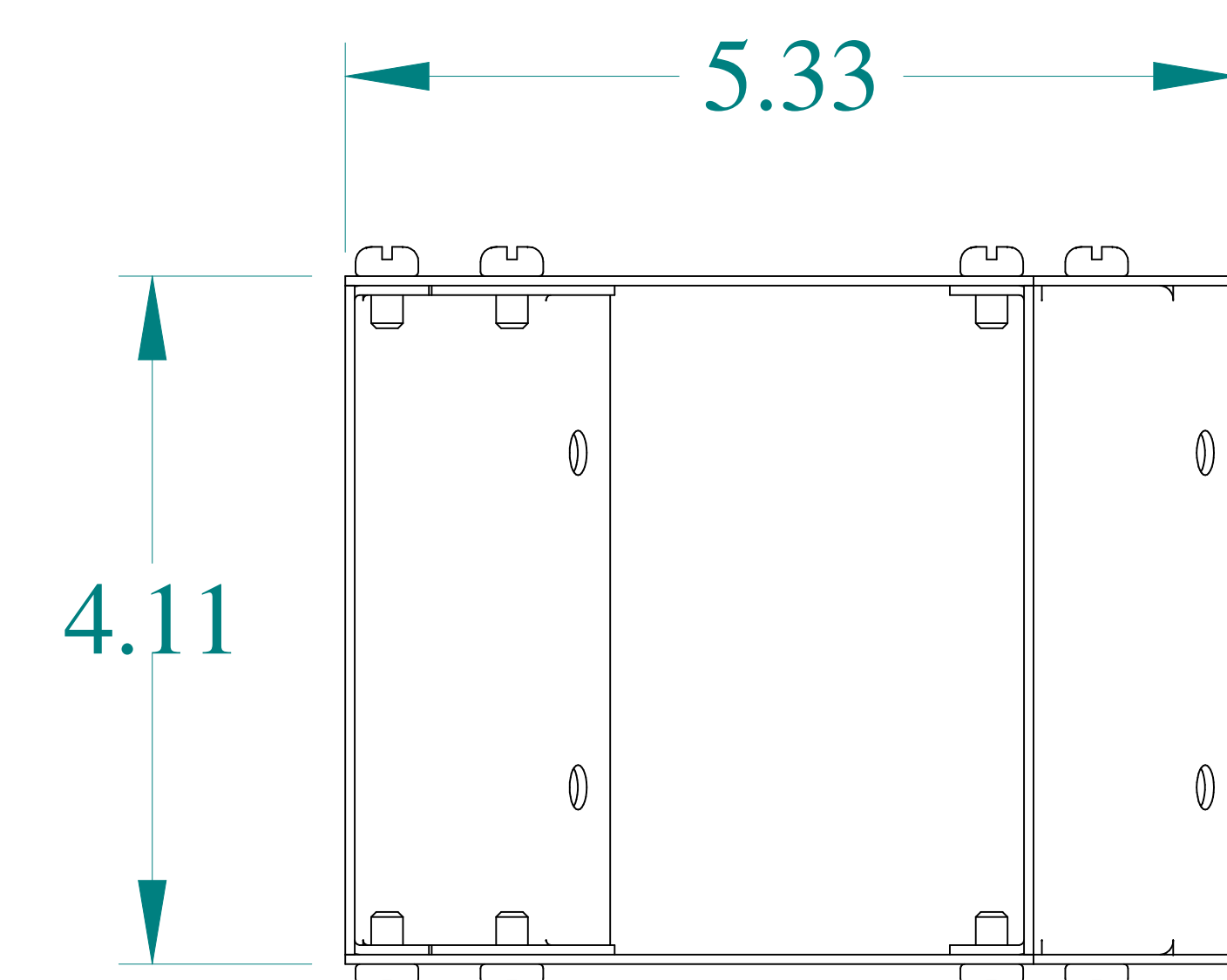
FRONT VIEW
