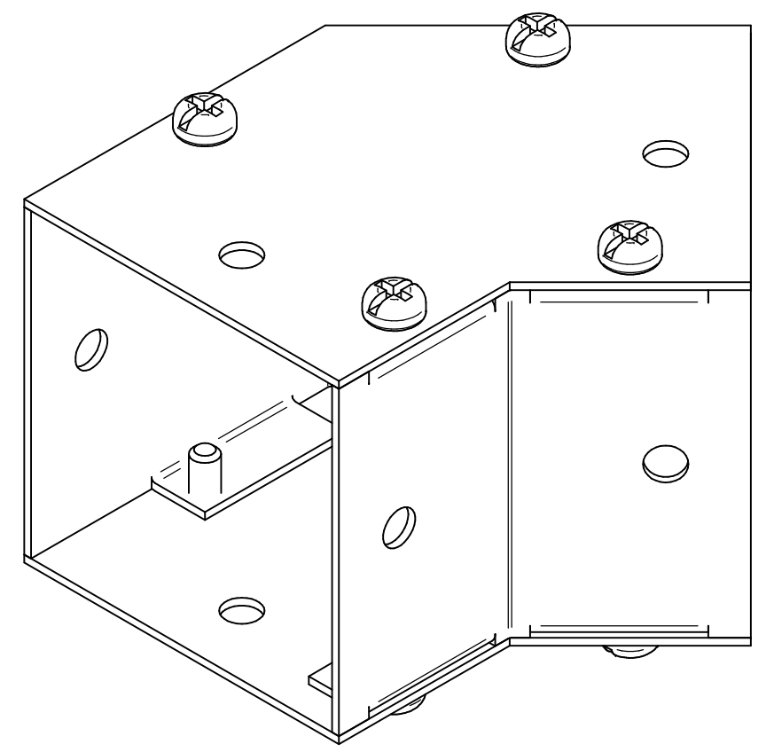
ISOMETRIC VIEWS
