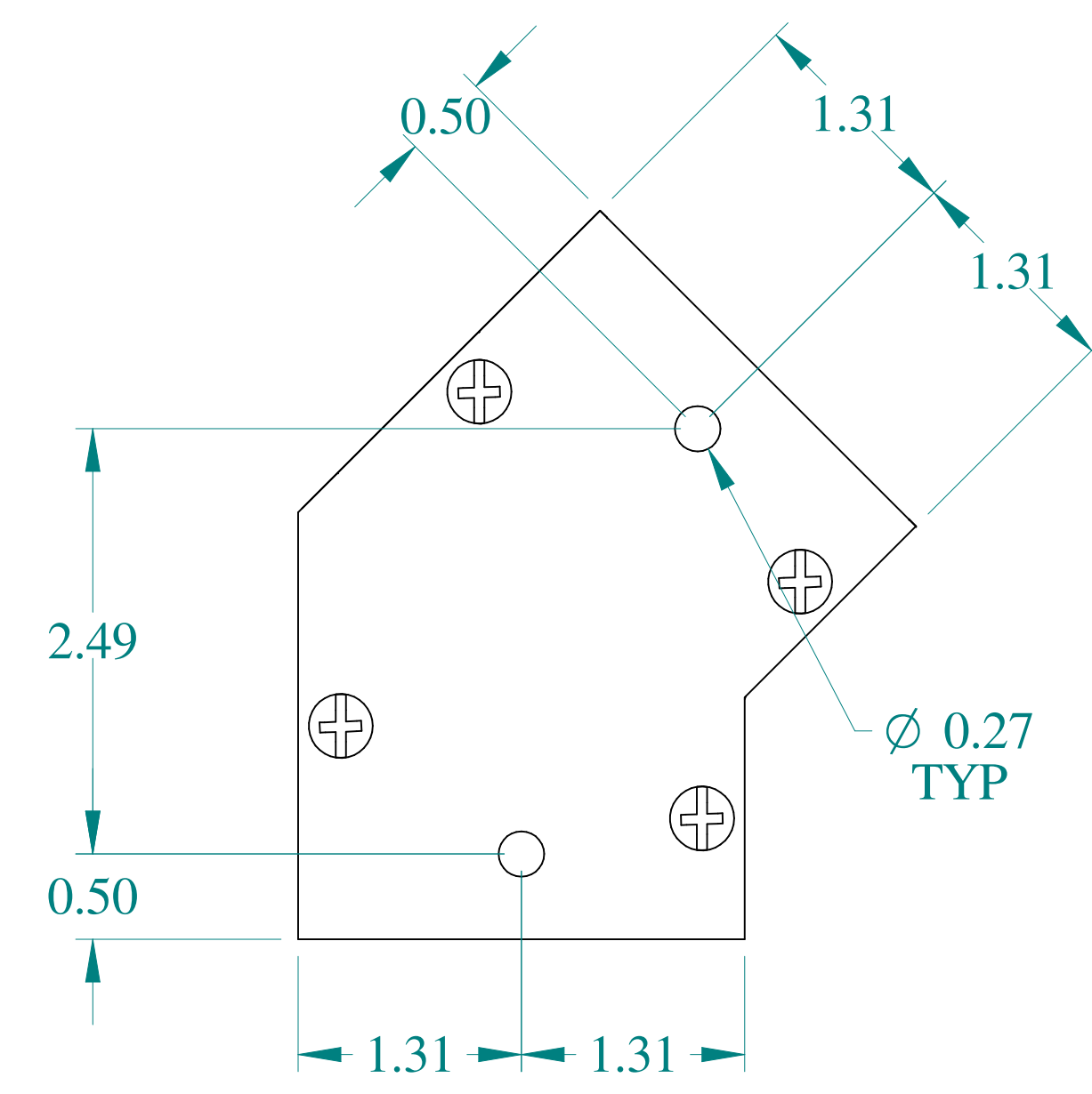
TOP VIEW
