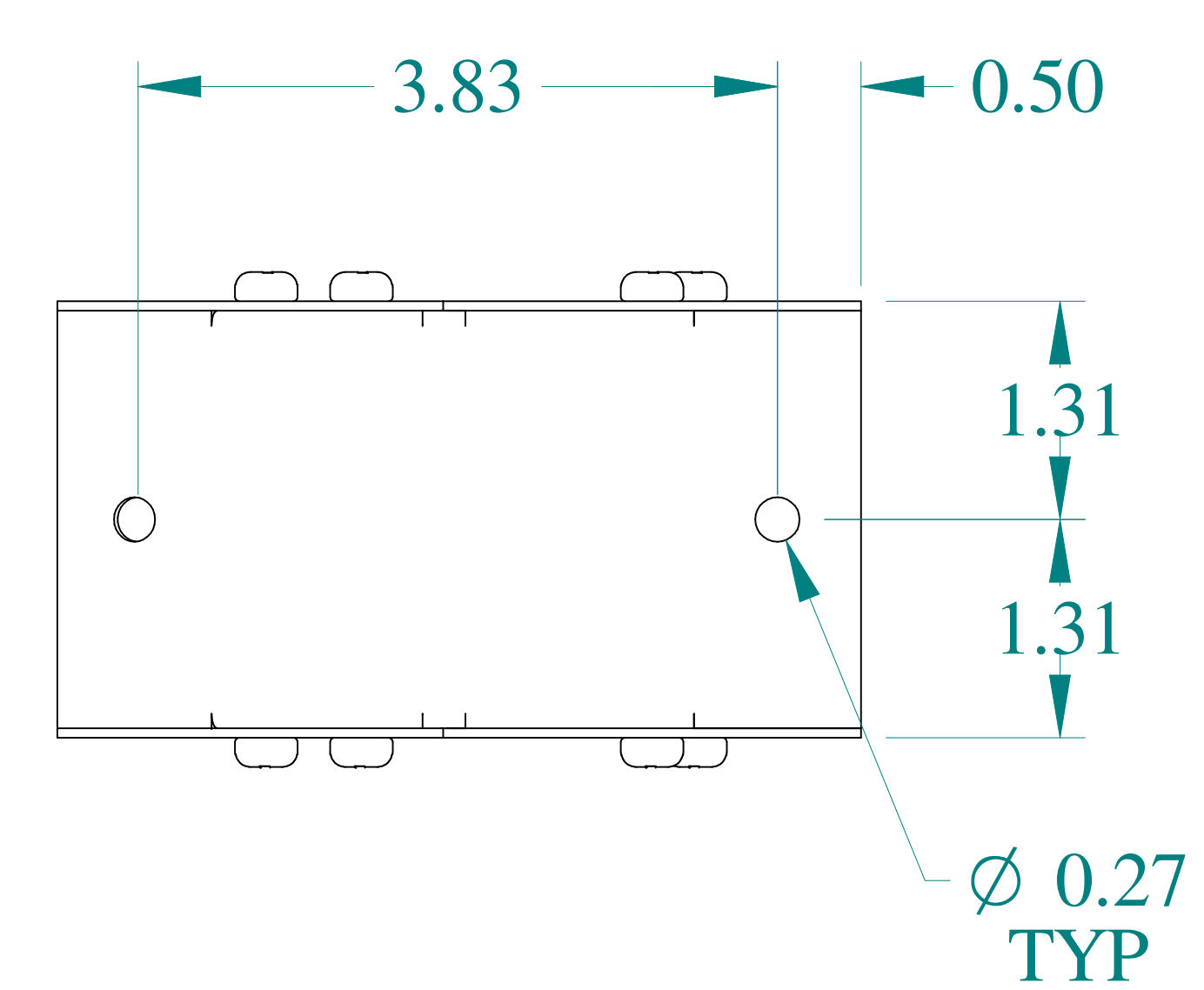
SIDE VIEW
