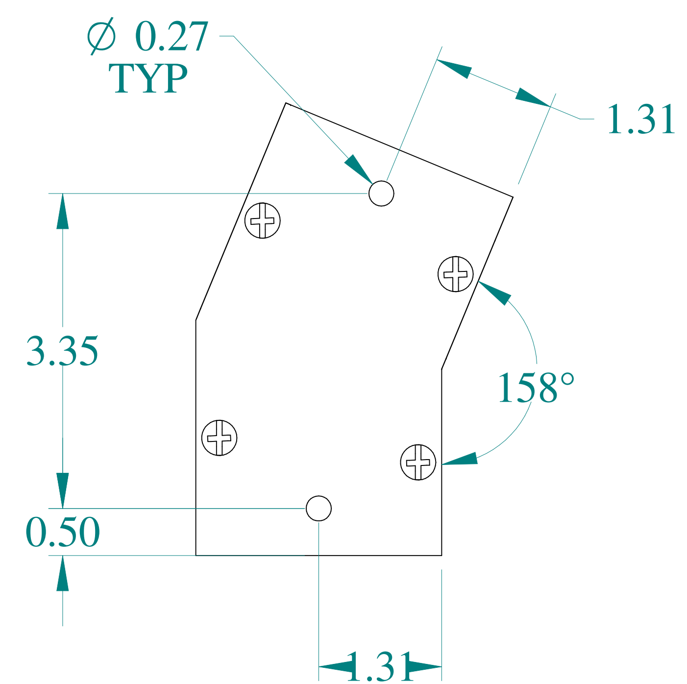
TOP VIEW
