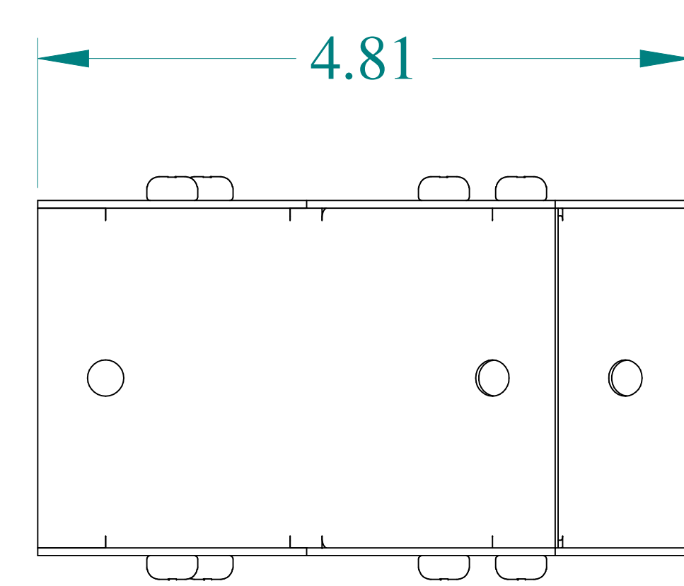
SIDE VIEW
