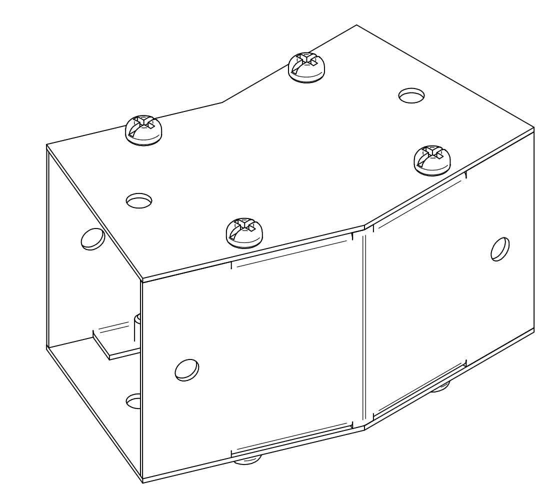
ISOMETRIC VIEWS
