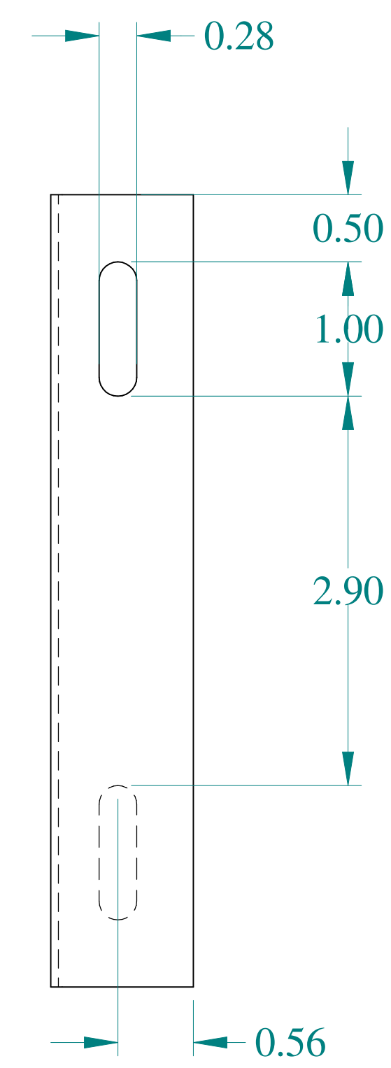
SIDE VIEW
