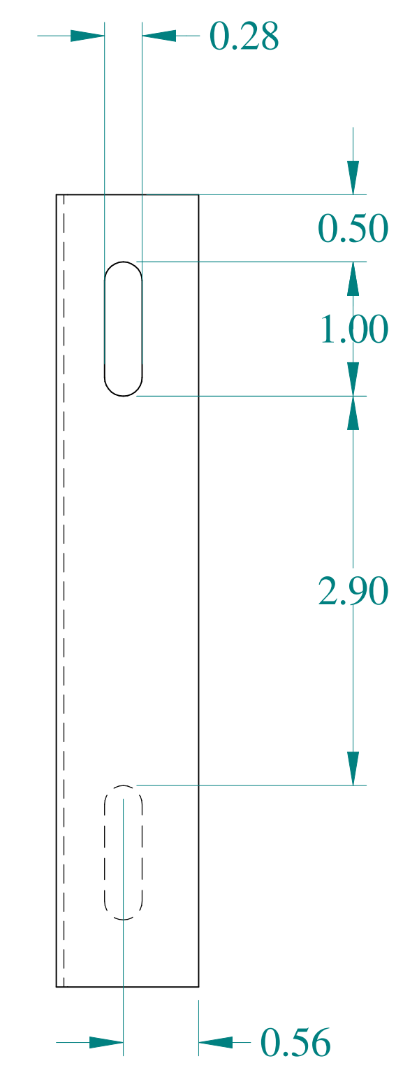
SIDE VIEW
