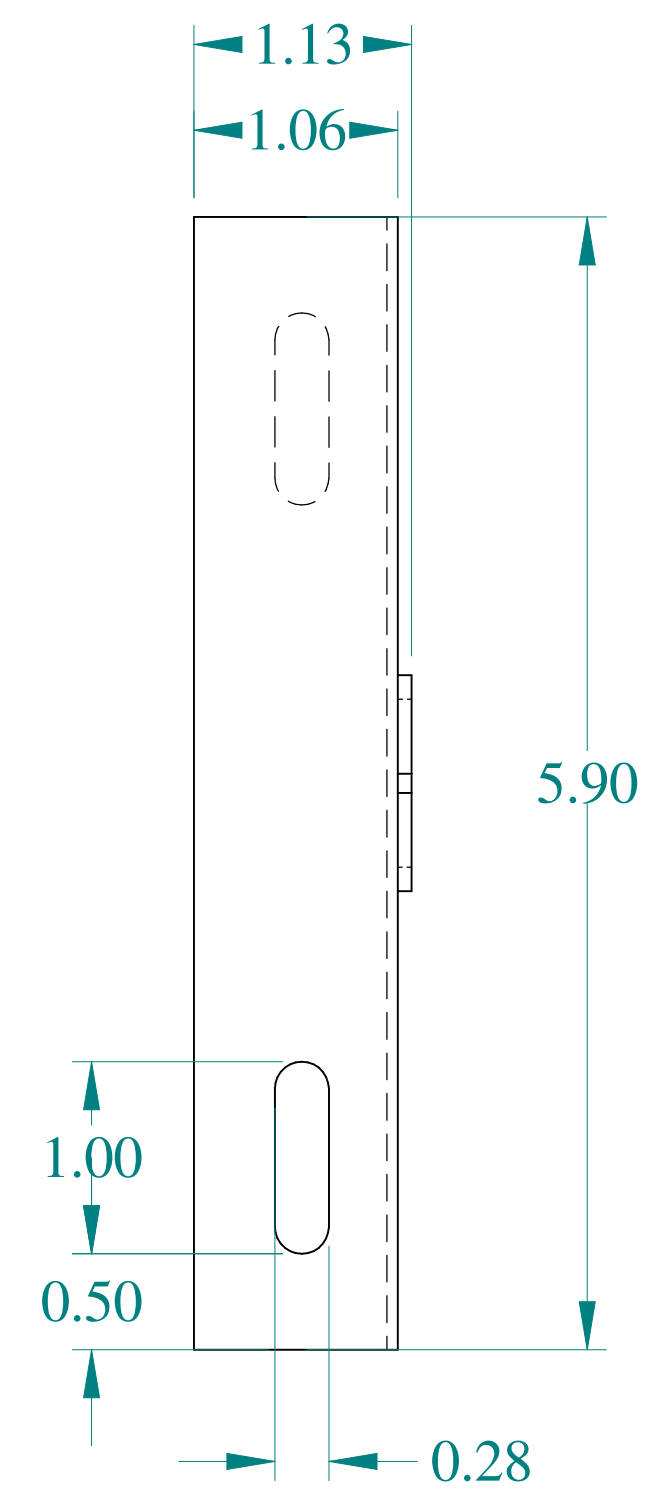
SIDE VIEW
