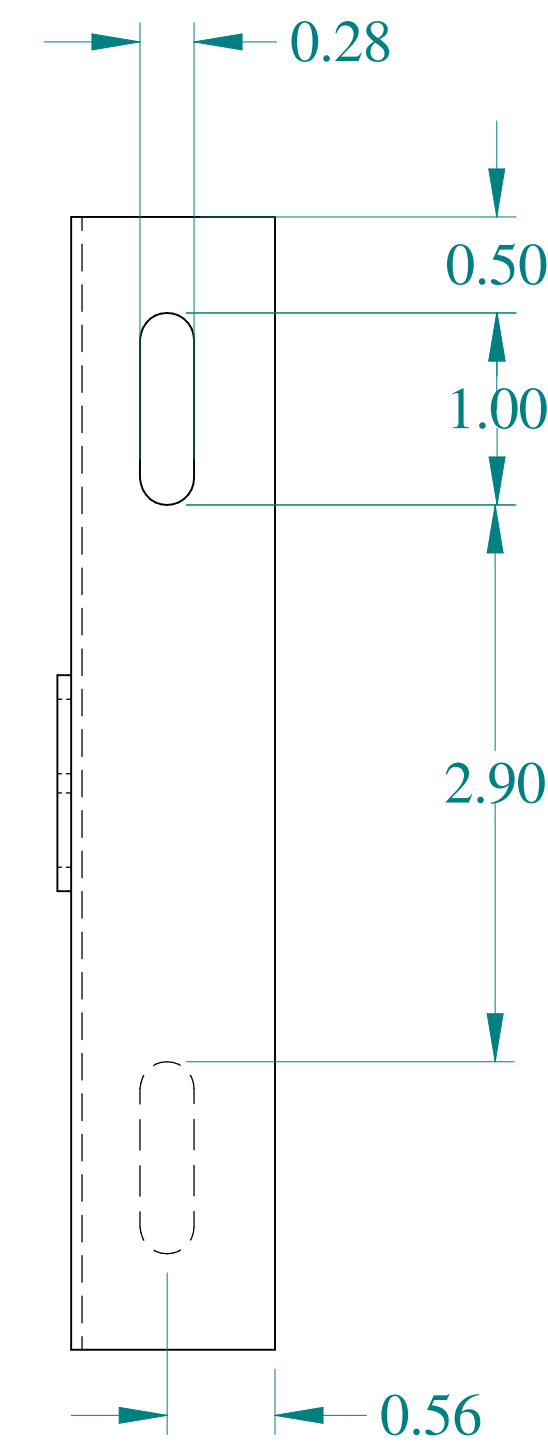
SIDE VIEW
