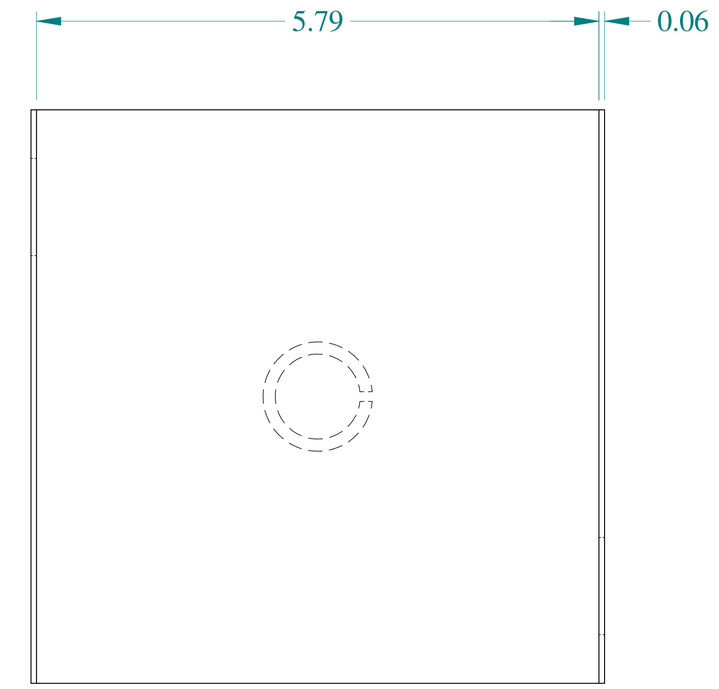
BACK VIEW
