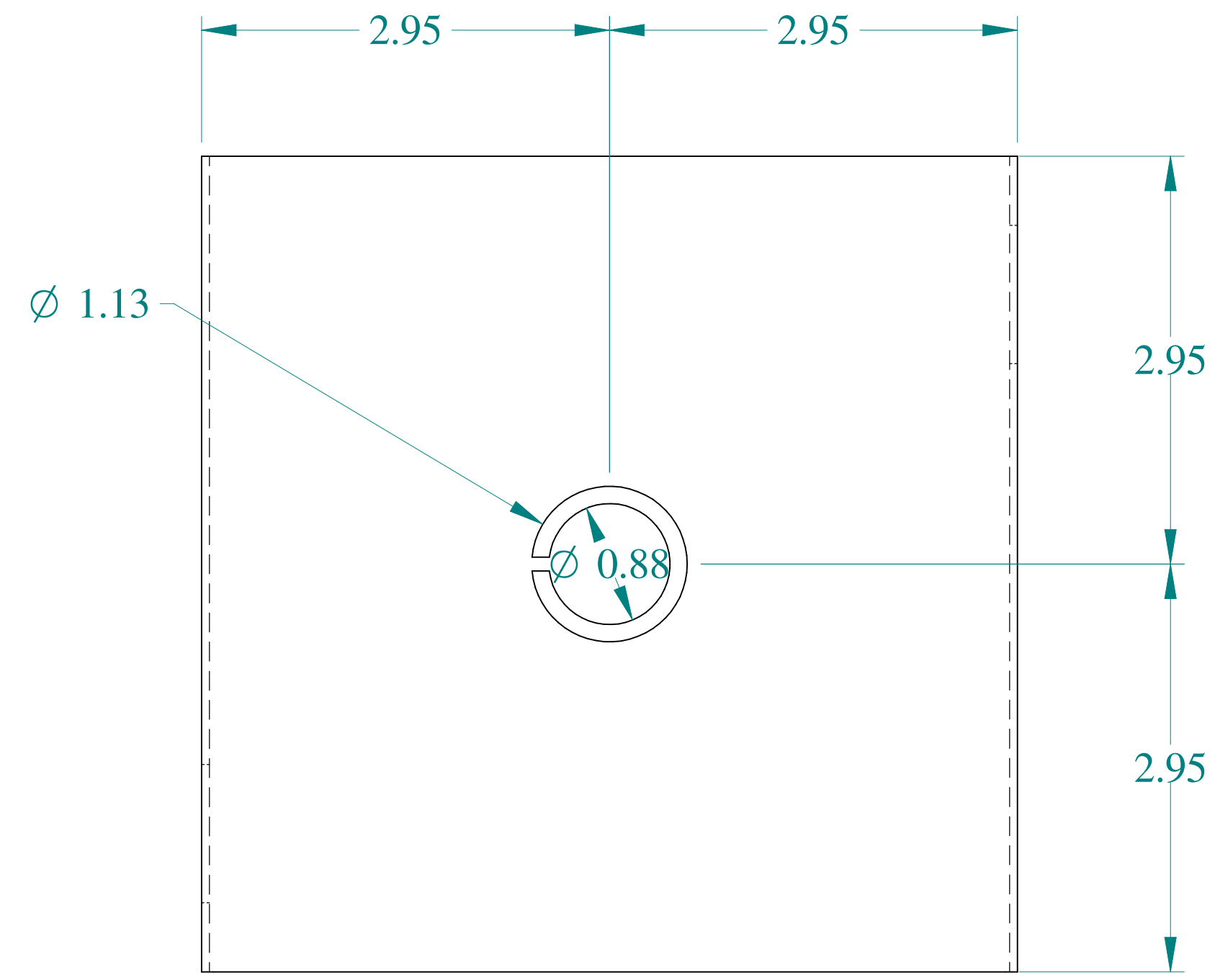
FRONT VIEW
