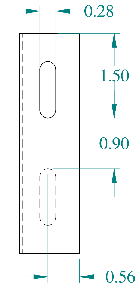
SIDE VIEW
