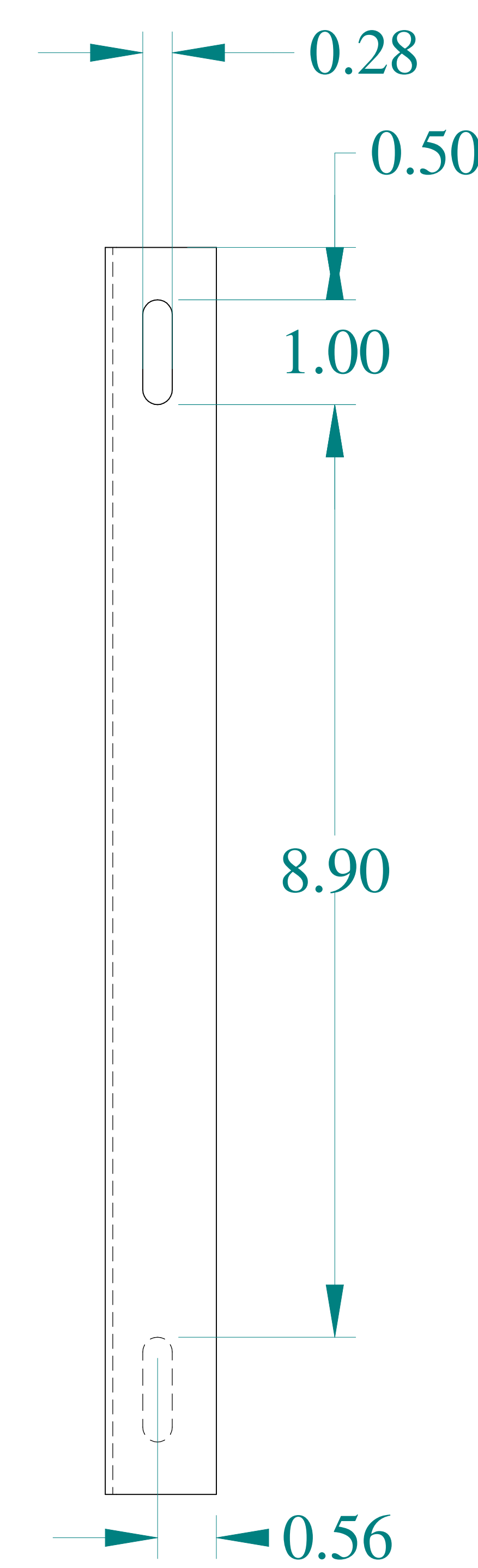
SIDE VIEW
