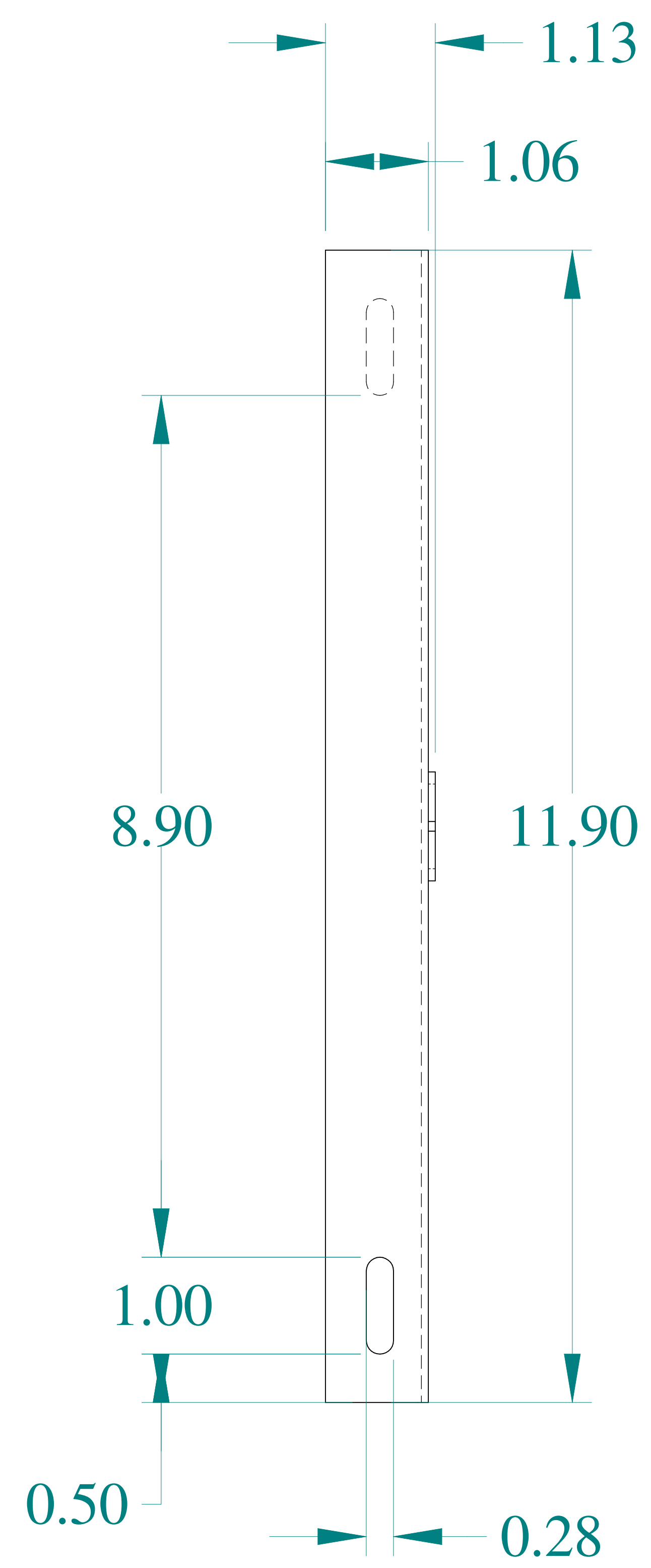
SIDE VIEW
