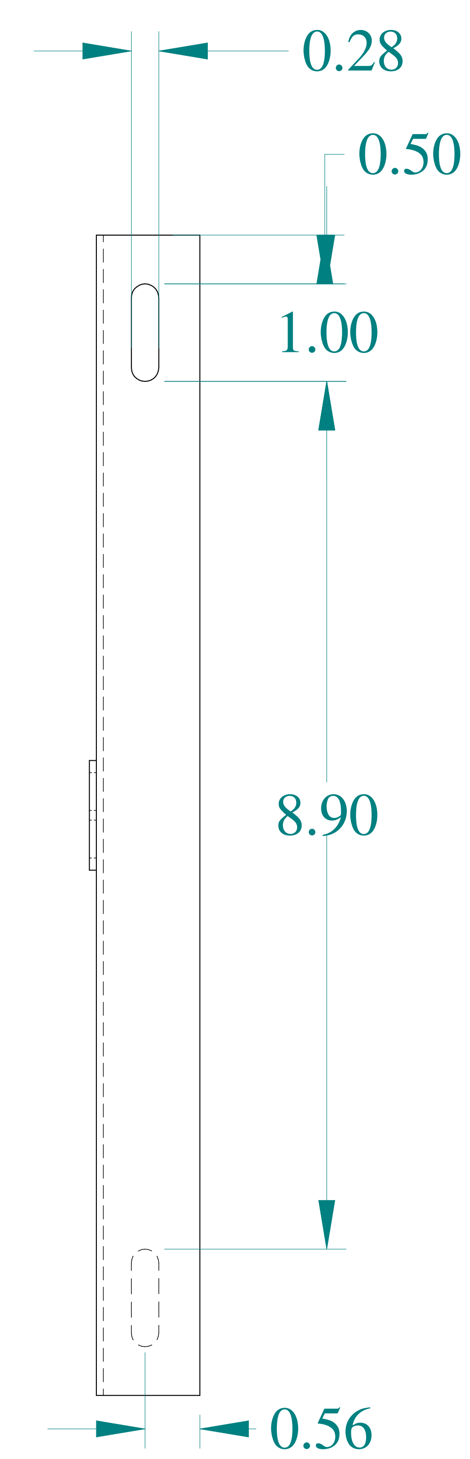
SIDE VIEW
