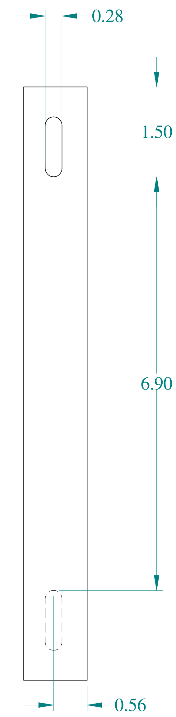
SIDE VIEW
